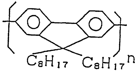
COMPOUND 1
