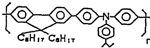
COMPOUND 2
