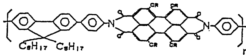
COMPOUND 5
