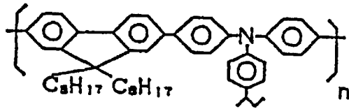
COMPOUND 2
