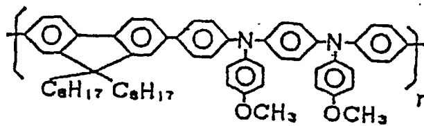
COMPOUND 3
