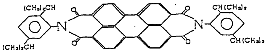
COMPOUND 8
