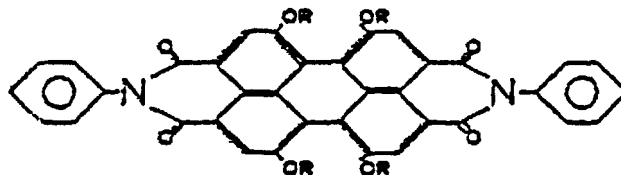
COMPOUND 6
