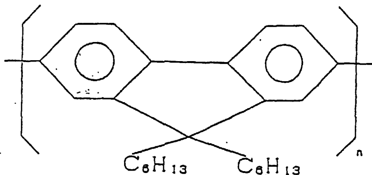
COMPOUND 7
