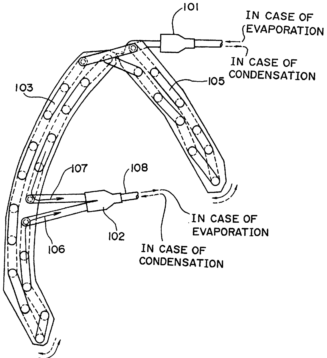
Fig.6 PRIOR ART
