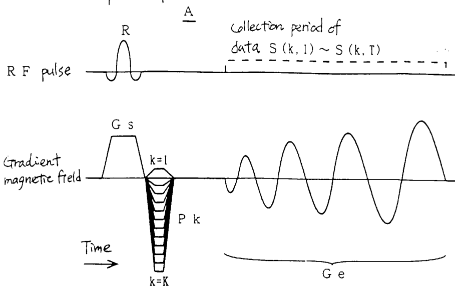
FIG. 6 Gradient magnetic field measurement pulse sequence
