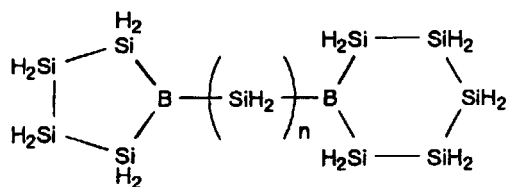
Compound 9
