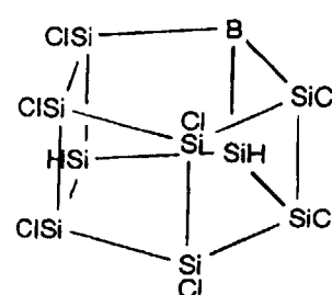
Compound 23
