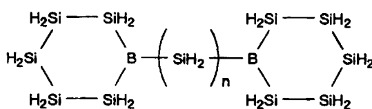
Compound 10
