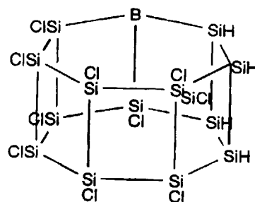
Compound 25
