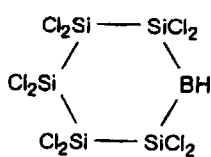
Compound 17
