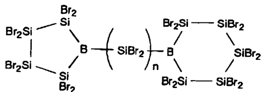
Compound 19
