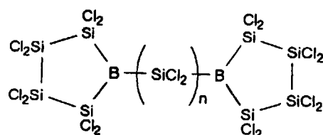
Compound 18
