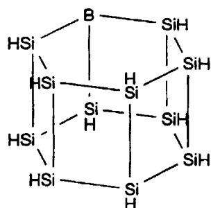
Compound 14
