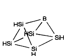
Compound 11
