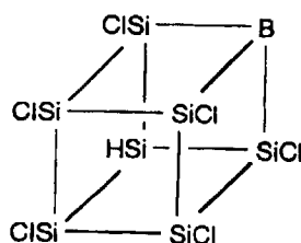
Compound 22
