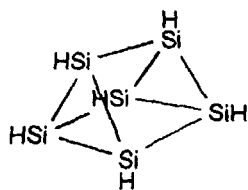
Compound 1
