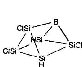
Compound 21
