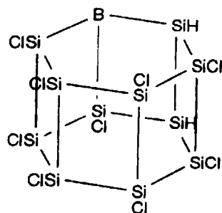
Compound 24
