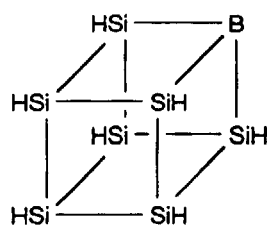
Compound 12
