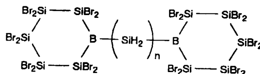
Compound 20
