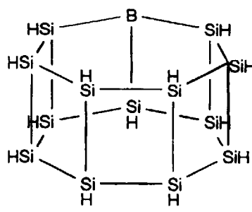
Compound 15
