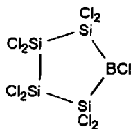
Compound 16
