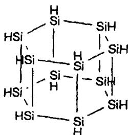
Compound 4
