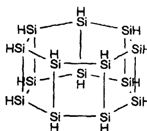
Compound 5
