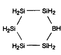
Compound 7
