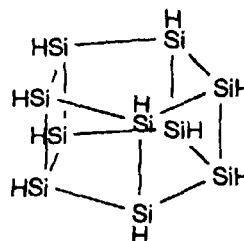
Compound 3
