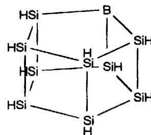
Compound 13
