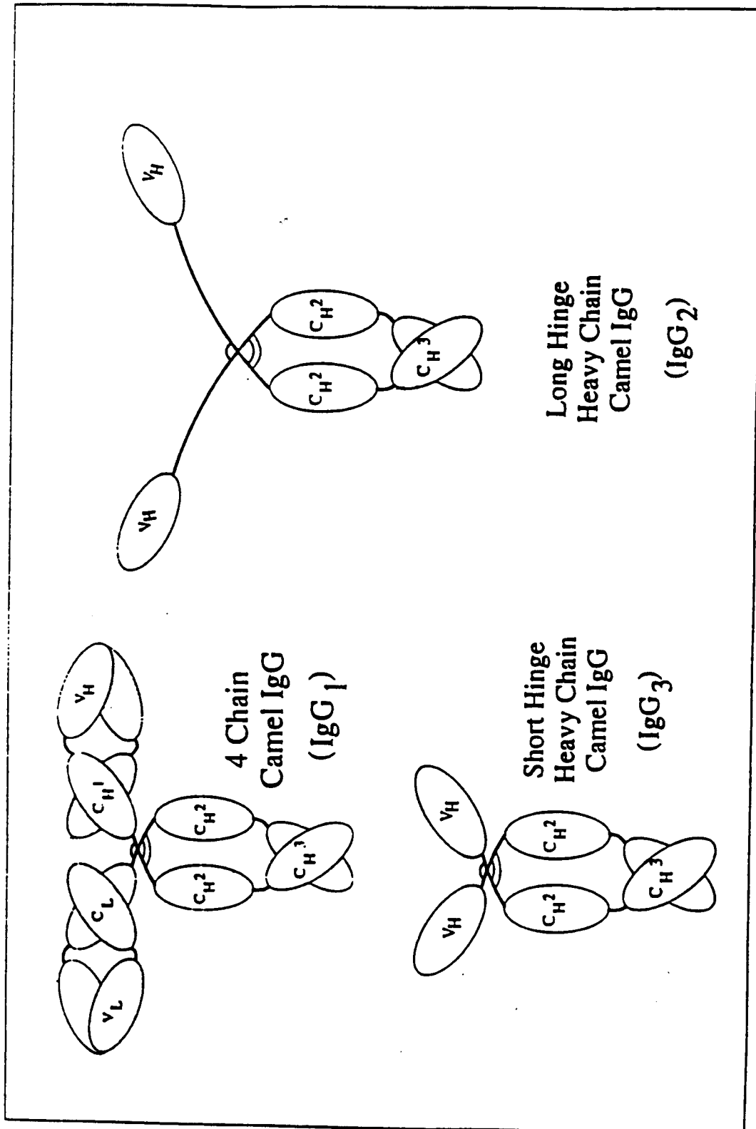
Fig 6: A schematic representation of Camel immunoglobulins IgG 1 , the putative IgG 2 and IgG 3 . The large (Pro-X) 12 of the putative IgG 2 molecule can be modelled into a 6 aa repeat
