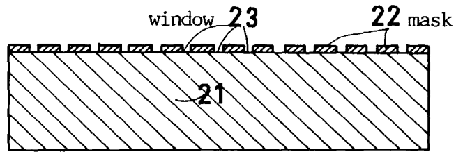
Fig.21 (a) manufacturing process of GaN substrate Embodiment 5
