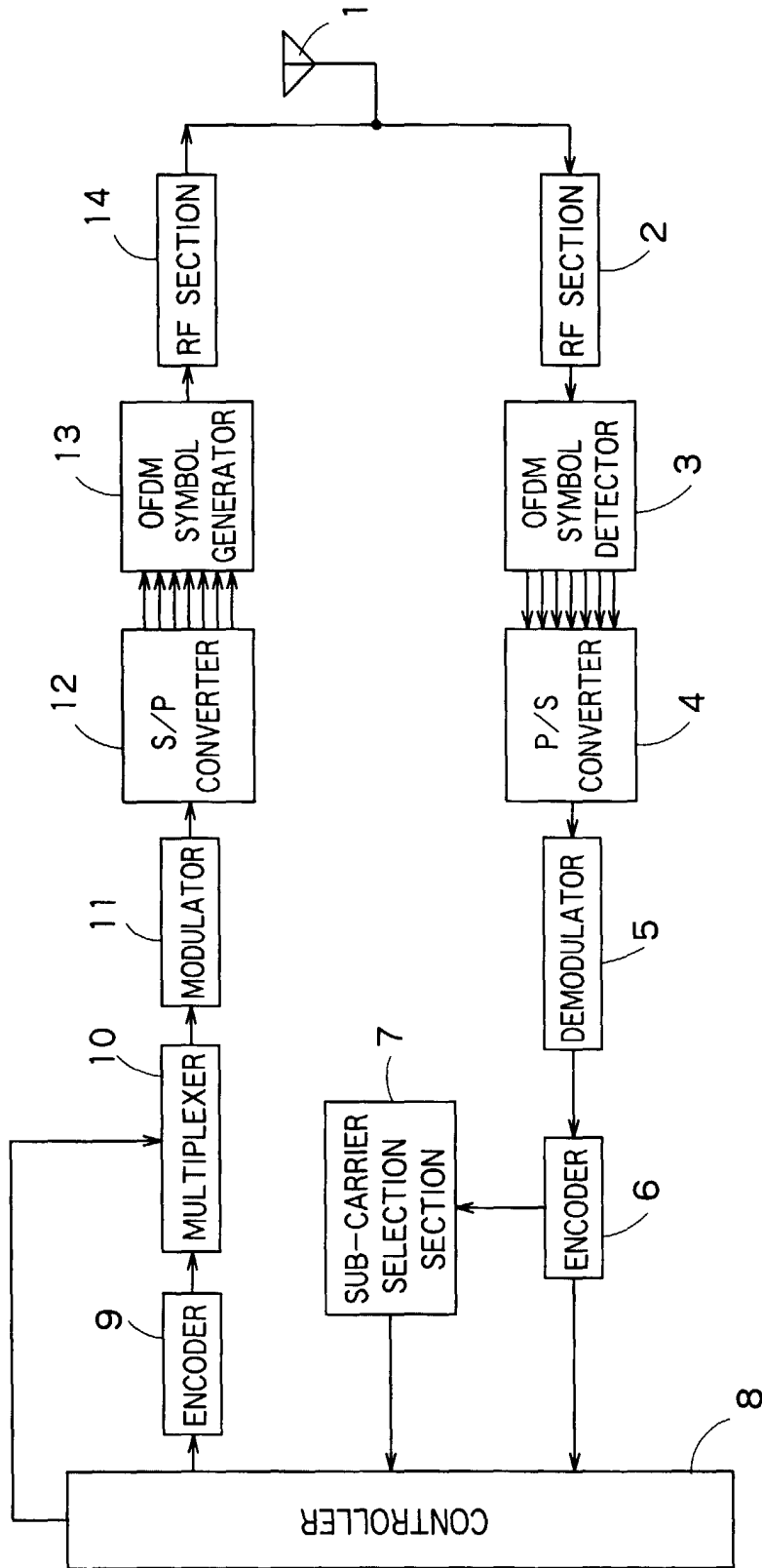
TERMINAL STATION CONSTITUTION
