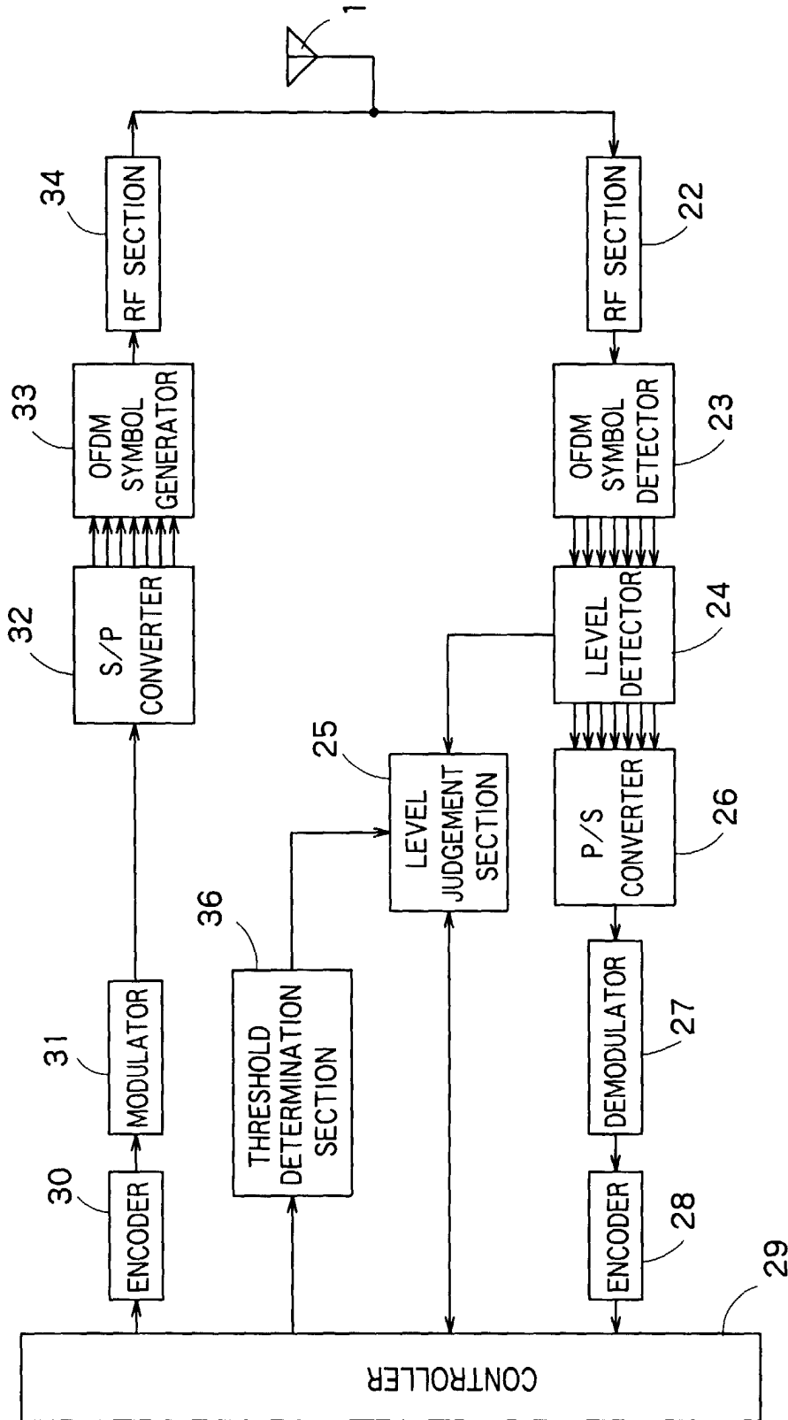
BASE STATION CONSTITUTION
