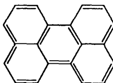
perylene
