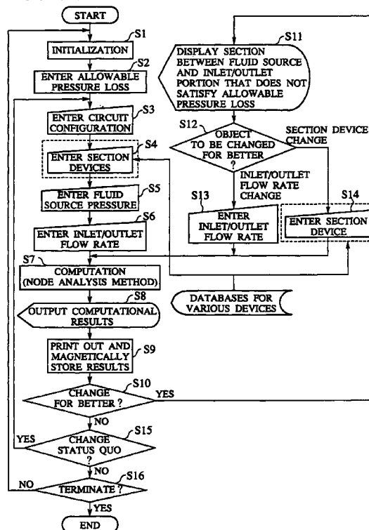
FIG.1 FLOW OF FLUID PIPELINE NETWORK DEVICE SELECTING METHOD
