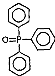
(II-5)
