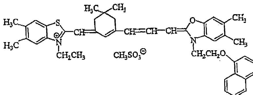
Compound B
