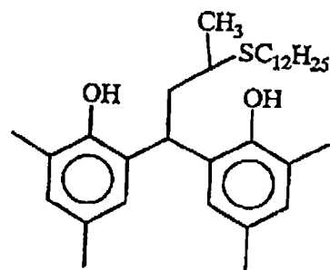
(I-21)
