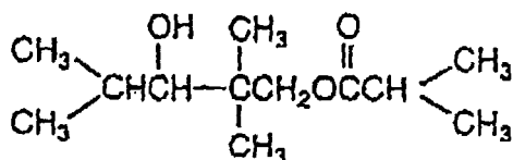
Compound E
