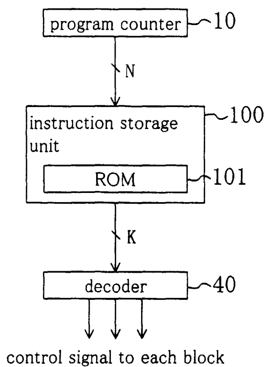
Fig. 11 PRIOR ART
