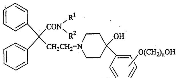
Compound (1d)
