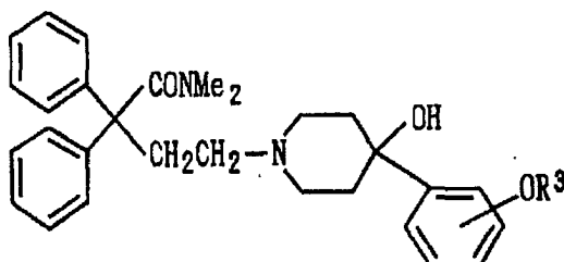
Compound List
