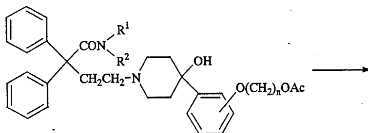
Compound (1c)
