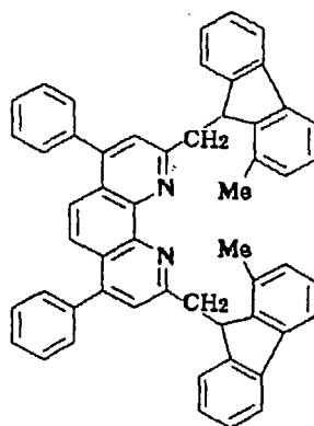
Compound No. 176
