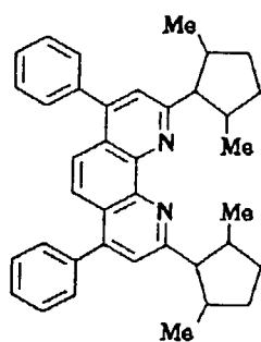
Compound No. 10
