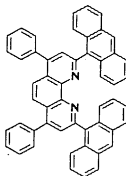
Compound No. 124
