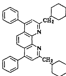
Compound No. 171
