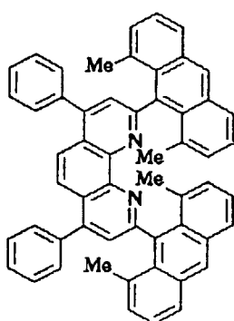
Compound No.127
