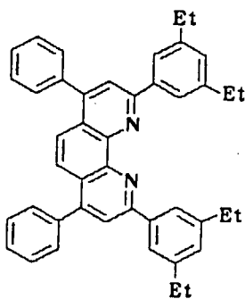
Compound No. 47
