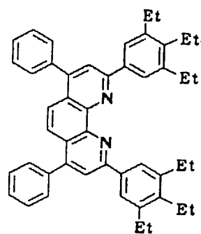
Compound No. 52
