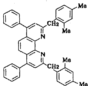
Compound No. 144
