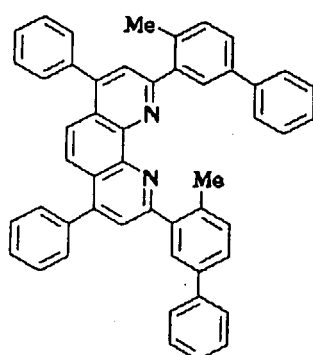
Compound No. 107
