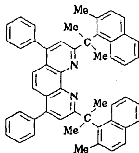
Compound No. 169
