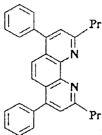
Compound No. 2
