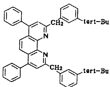
Compound No. 147
