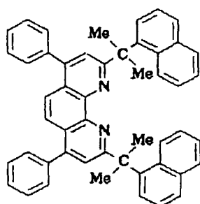
Compound No.167
