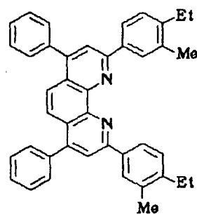
Compound No. 70
