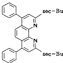
Compound No. 5
