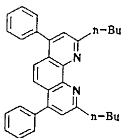
Compound No. 7
