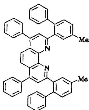
Compound No. 99
