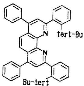
Compound No. 53
