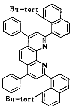
Compound No. 123
