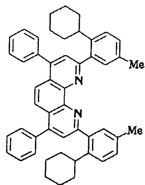
Compound No. 80
