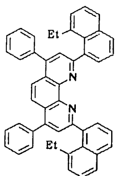
Compound No. 121
