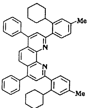
Compound No. 81
