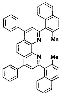
Compound No.126
