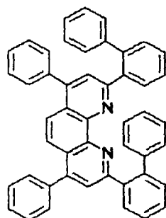
Compound No. 95
