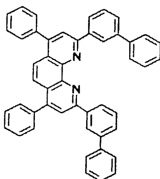
Compound No. 105
