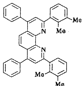
Compound No. 36
