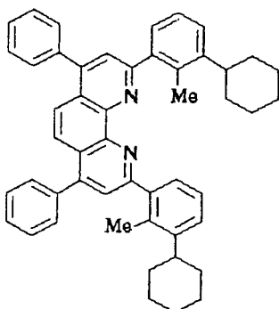
Compound No. 87
