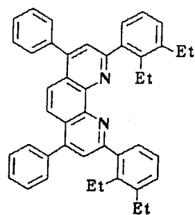
Compound No. 45
