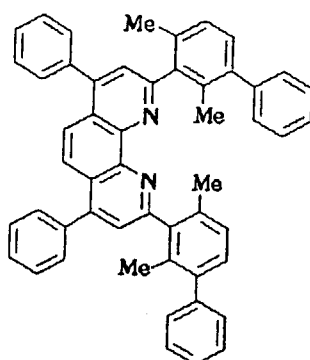
Compound No.109
