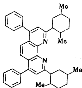
Compound No. 19
