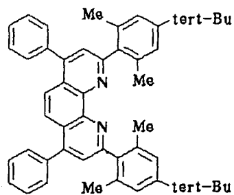
Compound No. 74
