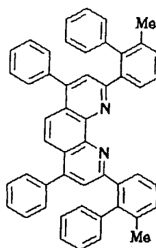
Compound No. 98
