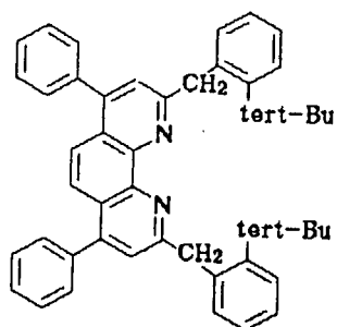
Compound No. 146
