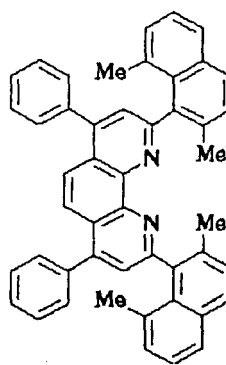
Compound No. 118
