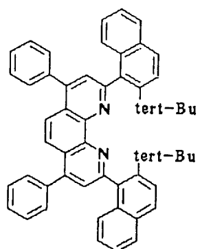
Compound No. 122
