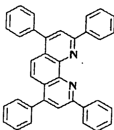
Compound No. 28
