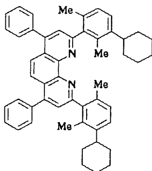
Compound No. 89
