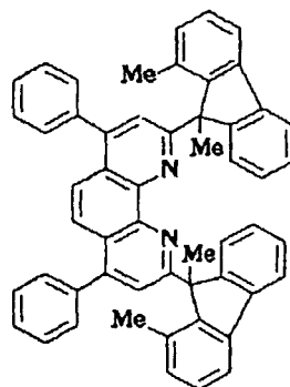
Compound No. 136
