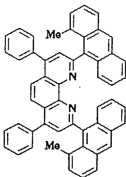
Compound No.125
