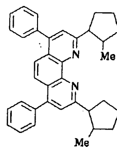
Compound No. 9
