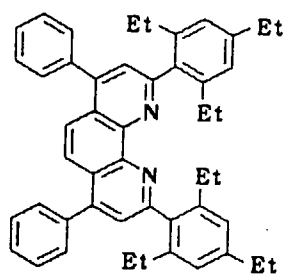
Compound No. 51
