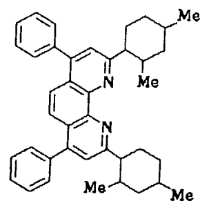
Compound No. 21
