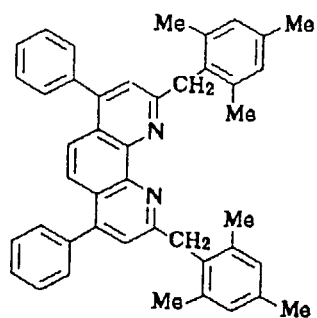
Compound No. 145
