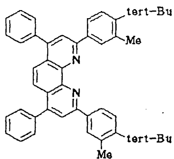
Compound No. 73
