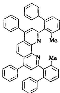
Compound No. 97
