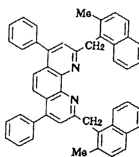
Compound No.162
