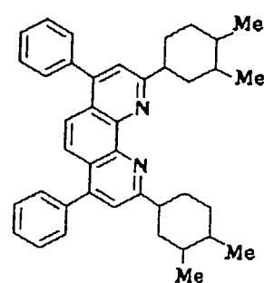
Compound No. 24
