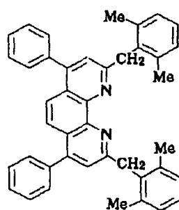
Compound No. 143
