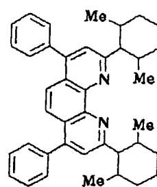
Compound No. 18
