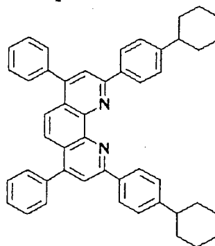
Compound No. 88
