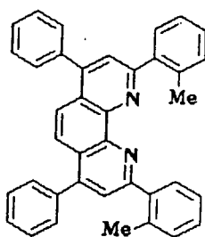
Compound No. 29
