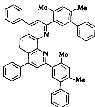
Compound No.111
