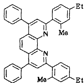
Compound No. 68
