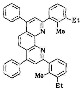
Compound No. 67
