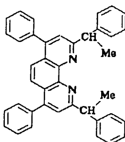
Compound No. 139
