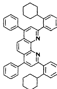
Compound No. 78
