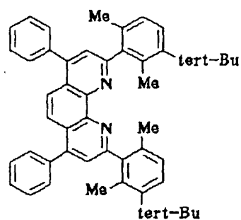
Compound No. 76
