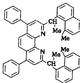
Compound No.164
