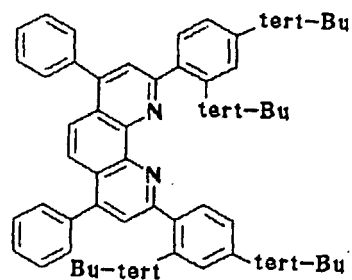
Compound No. 59
