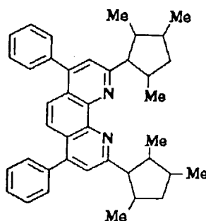
Compound No. 11
