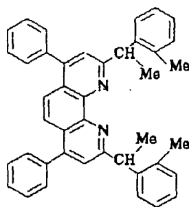
Compound No. 142
