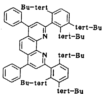
Compound No. 64
