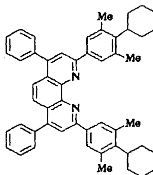
Compound No. 94
