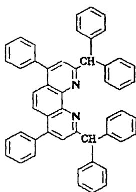
Compound No. 159
