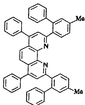
Compound No. 100
