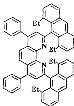
Compound No. 130
