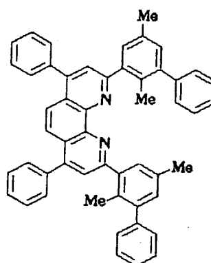
Compound No.112
