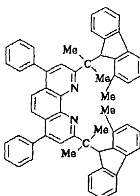
Compound No. 178
