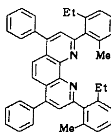
Compound No. 66
