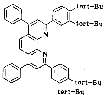
Compound No. 61
