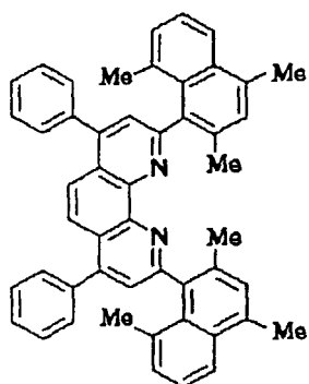
Compound No. 119
