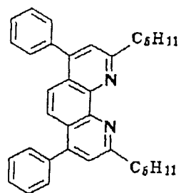
Compound No. 13
