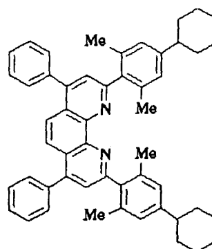
Compound No. 92
