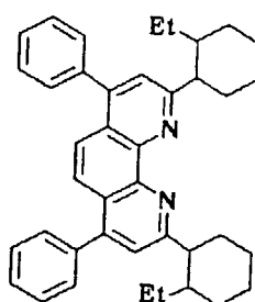
Compound No. 20
