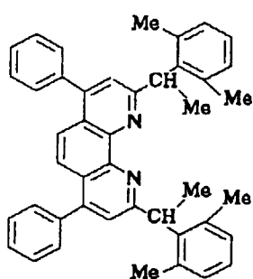
Compound No. 151
