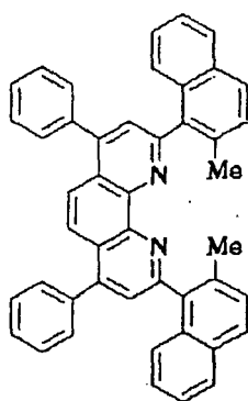
Compound No. 117
