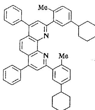
Compound No. 86
