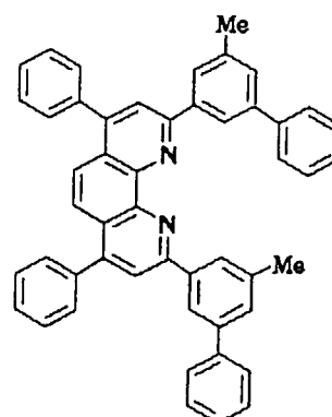
Compound No. 108
