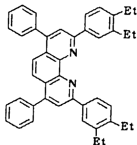
Compound No. 48
