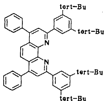
Compound No. 60
