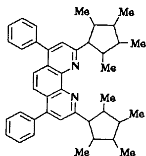
Compound No. 12
