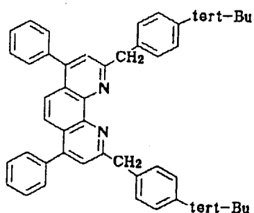
Compound No. 148
