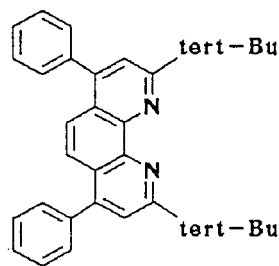
Compound No. 6
