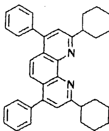
Compound No. 14
