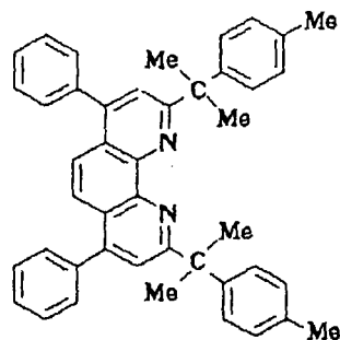
Compound No. 158
