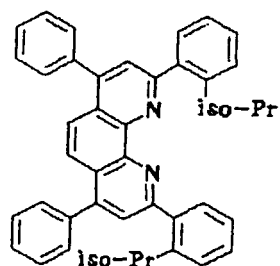
Compound No. 57
