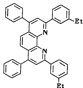
Compound No. 42
