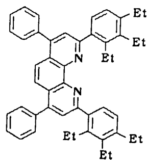
Compound No. 50
