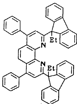
Compound No. 137
