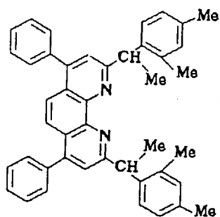
Compound No. 153
