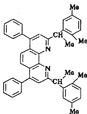
Compound No. 152
