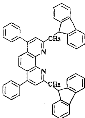
Compound No. 173
