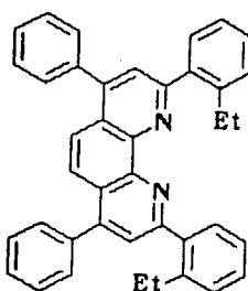
Compound No. 41
