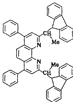
Compound No. 174
