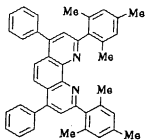
Compound No. 39
