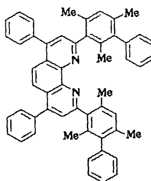
Compound No. 114
