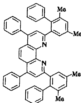
Compound No. 102
