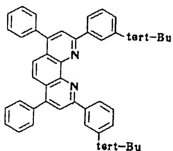
Compound No. 54
