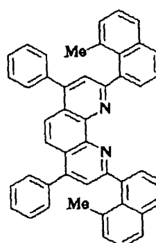
Compound No. 116
