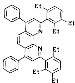
Compound No. 49
