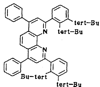
Compound No. 58
