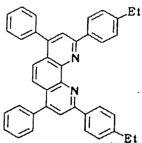
Compound No. 43
