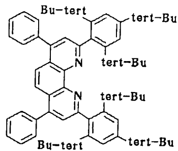
Compound No. 62
