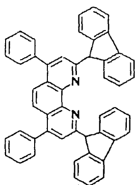
Compound No. 133
