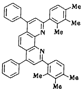
Compound No. 38
