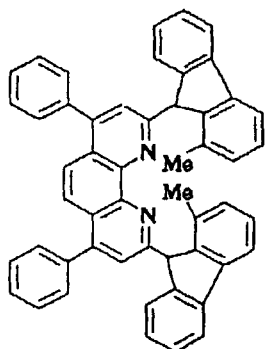
Compound No. 135
