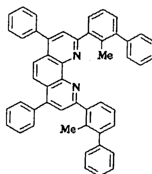
Compound No. 106
