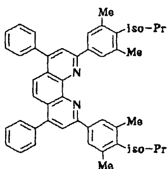
Compound No. 77
