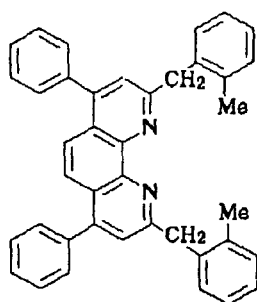
Compound No. 141
