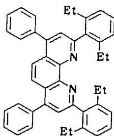
Compound No. 44
