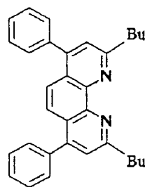
Compound No. 4
