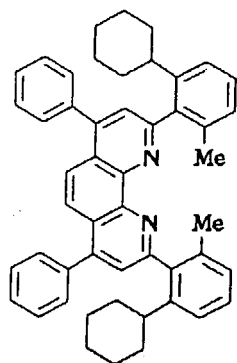
Compound No. 79
