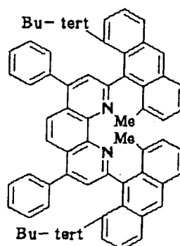
Compound No. 132
