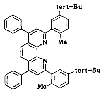
Compound No. 70
