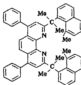
Compound No.168
