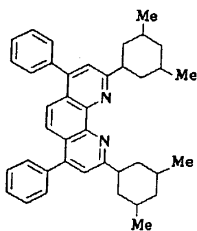
Compound No. 23
