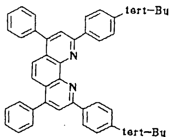
Compound No. 55
