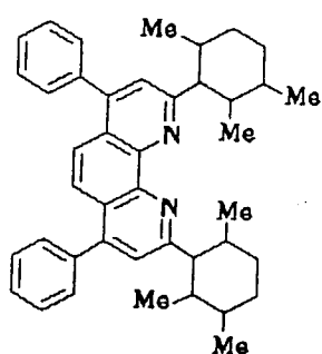
Compound No. 25
