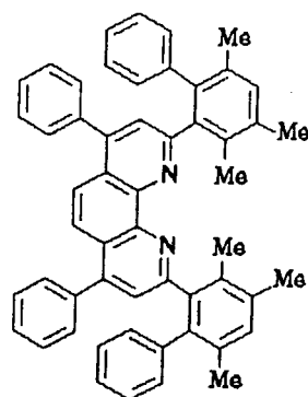
Compound No. 104
