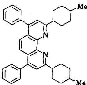
Compound No. 17
