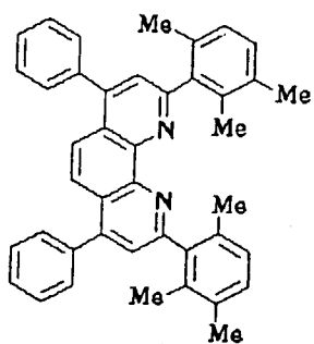
Compound No. 37
