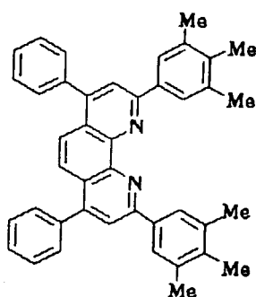
Compound No. 40
