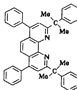
Compound No. 140
