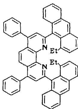
Compound No. 129
