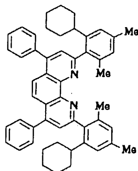
Compound No. 84
