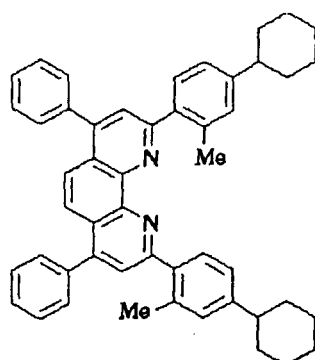
Compound No. 91
