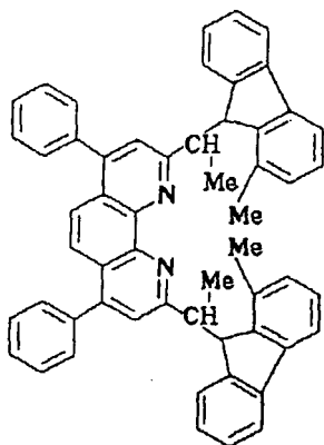
Compound No. 177
