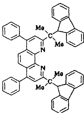
Compound No. 175
