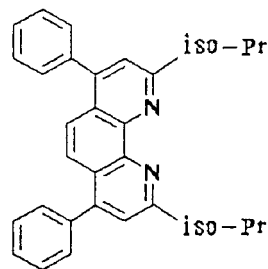
Compound No. 3
