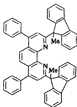
Compound No. 134
