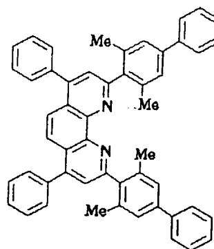
Compound No.110
