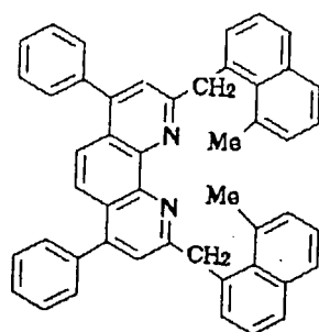
Compound No.161
