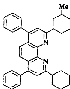
Compound No. 16
