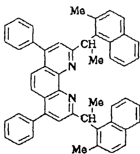
Compound No.165
