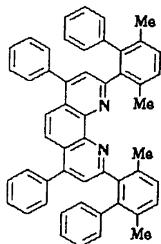
Compound No. 101
