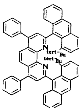
Compound No. 131
