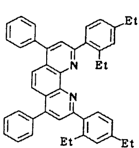
Compound No. 46
