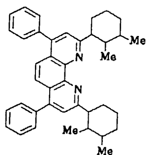
Compound No. 22
