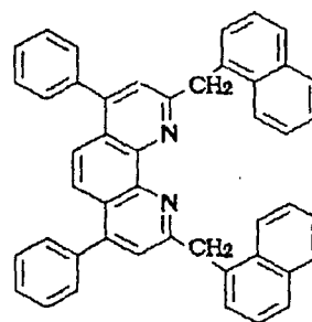
Compound No. 160
