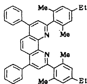
Compound No. 71
