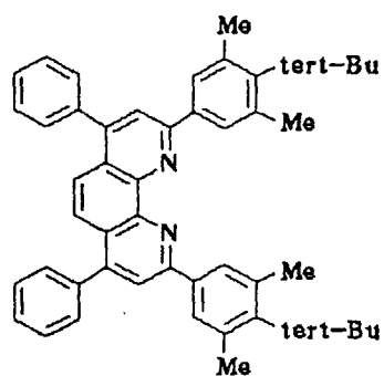
Compound No. 75
