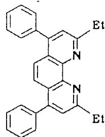
Compound No. 1
