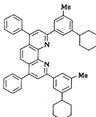
Compound No. 88
