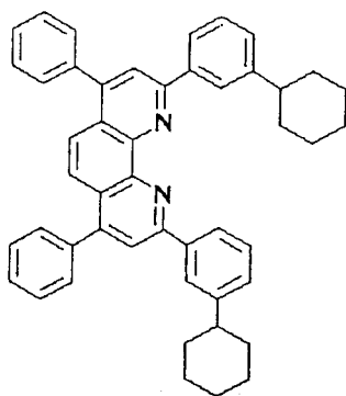
Compound No. 85
