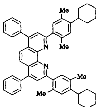
Compound No. 93
