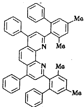
Compound No. 103
