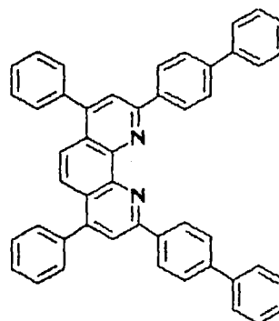
Compound No. 96
