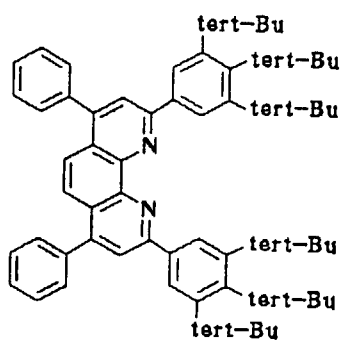
Compound No. 63
