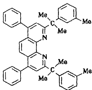
Compound No. 157
