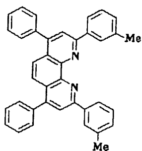
Compound No. 30
