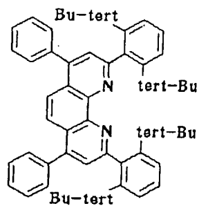
Compound No. 56
