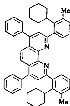
Compound No. 82
