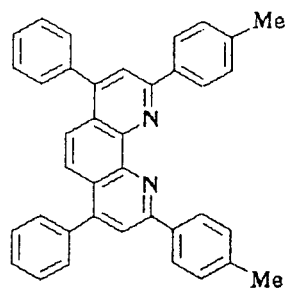
Compound No. 31
