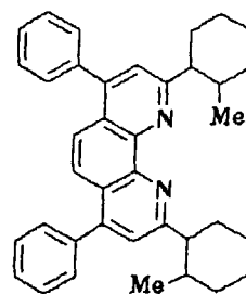
Compound No. 15
