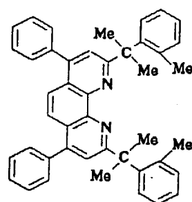
Compound No. 156
