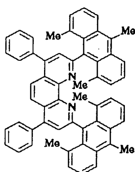
Compound No.128
