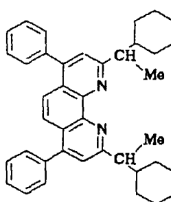
Compound No. 172
