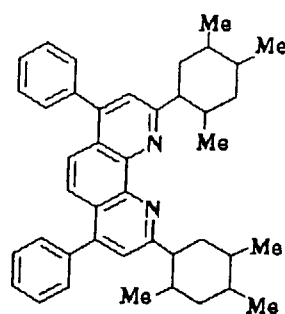
Compound No. 27
