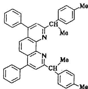
Compound No. 150
