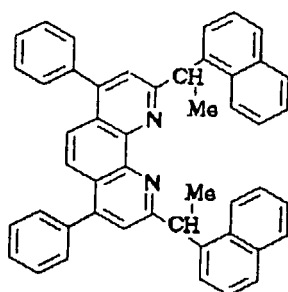
Compound No.163
