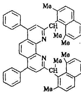
Compound No.166
