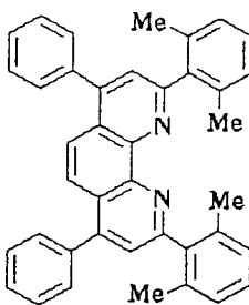
Compound No. 32
