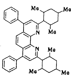
Compound No. 26
