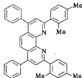
Compound No. 33
