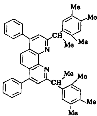
Compound No. 155
