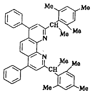
Compound No. 154
