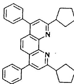
Compound No. 8
