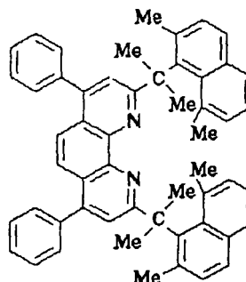
Compound No. 170
