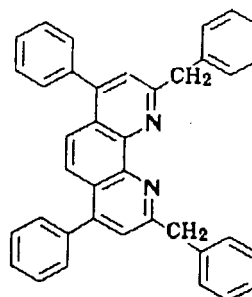
Compound No. 138
