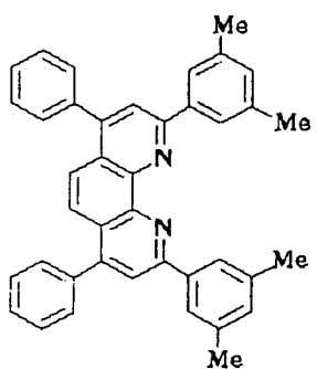
Compound No. 34
