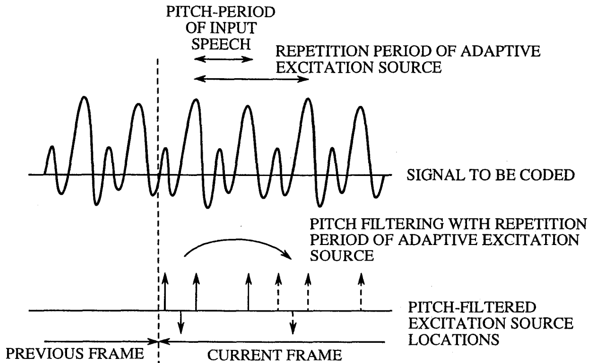
FIG.18 (PRIOR ART)
