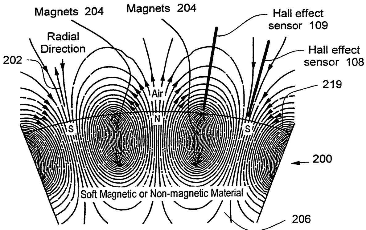
Magnetic Flux Lines on a Ring (3 poles shown)
