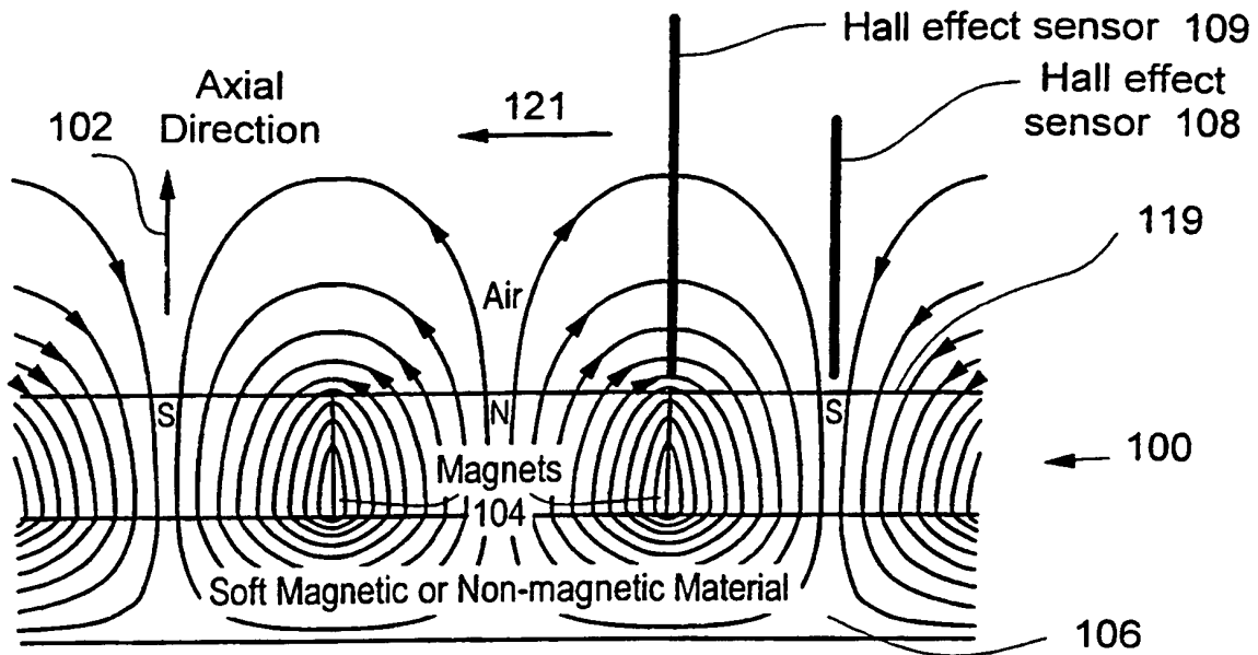
Magnetic Flux Lines on a Disk (3 poles shown)
