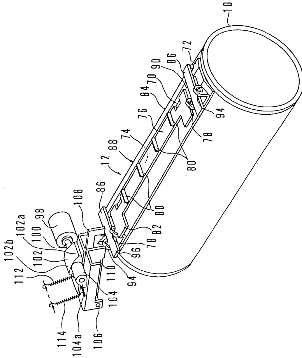
FIG. 2 PRIOR ART
