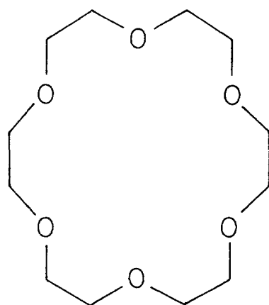
18-CROWN-6
