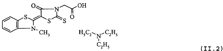
5-(3-methyl-3(3H)-benzothiazolylidene)-4-oxo-2-thioxo-3-thiazolidine acetic acid
