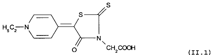
5-(1-ethyl-4(1H)-pyridylene)-4-oxo-2-thioxo-3-thiazolidine acetic acid
