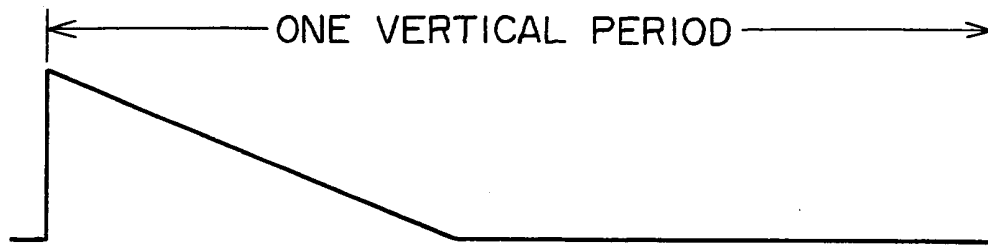
MODULATING CURRENT ( I_{v1} )
