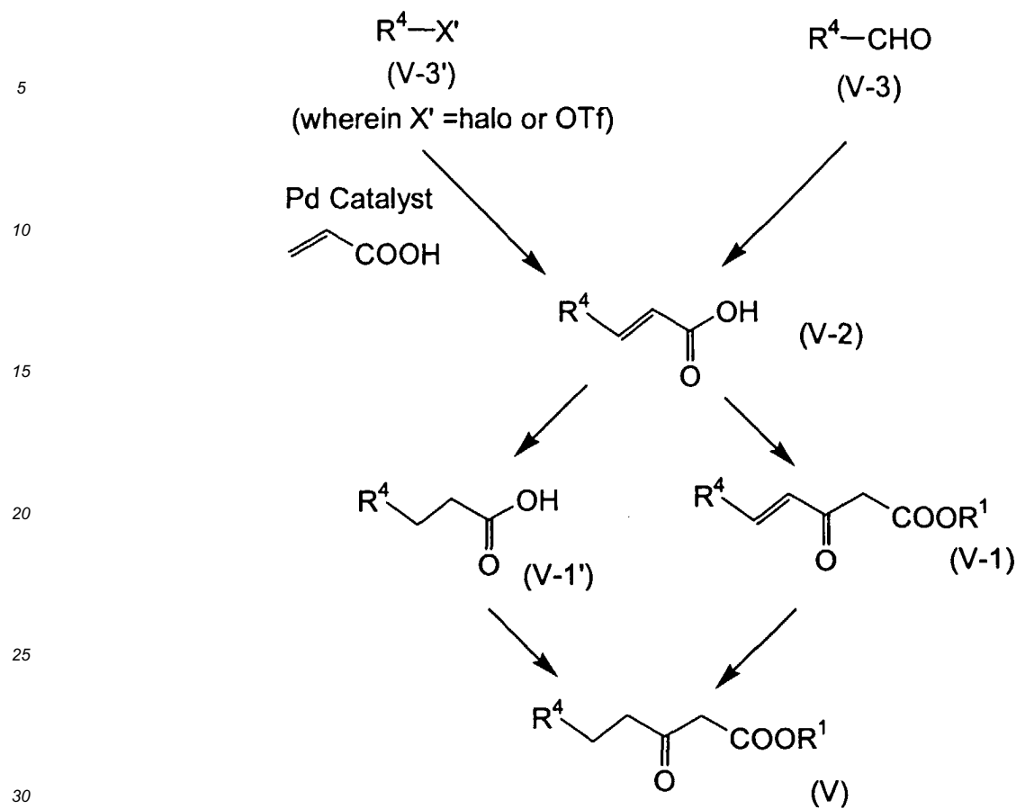
Scheme B-III-c
