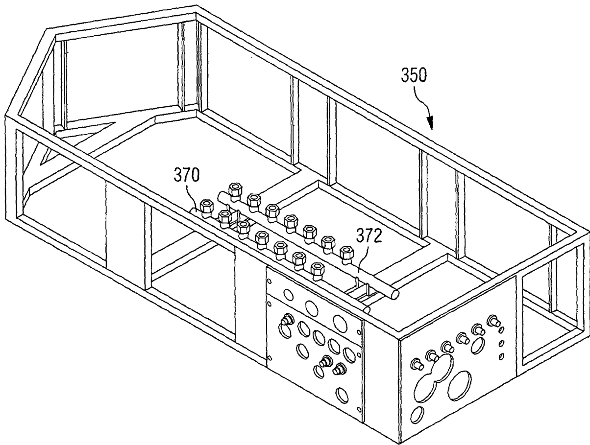
FIG 15 COOLING WATER SUPPLY & RETURN
