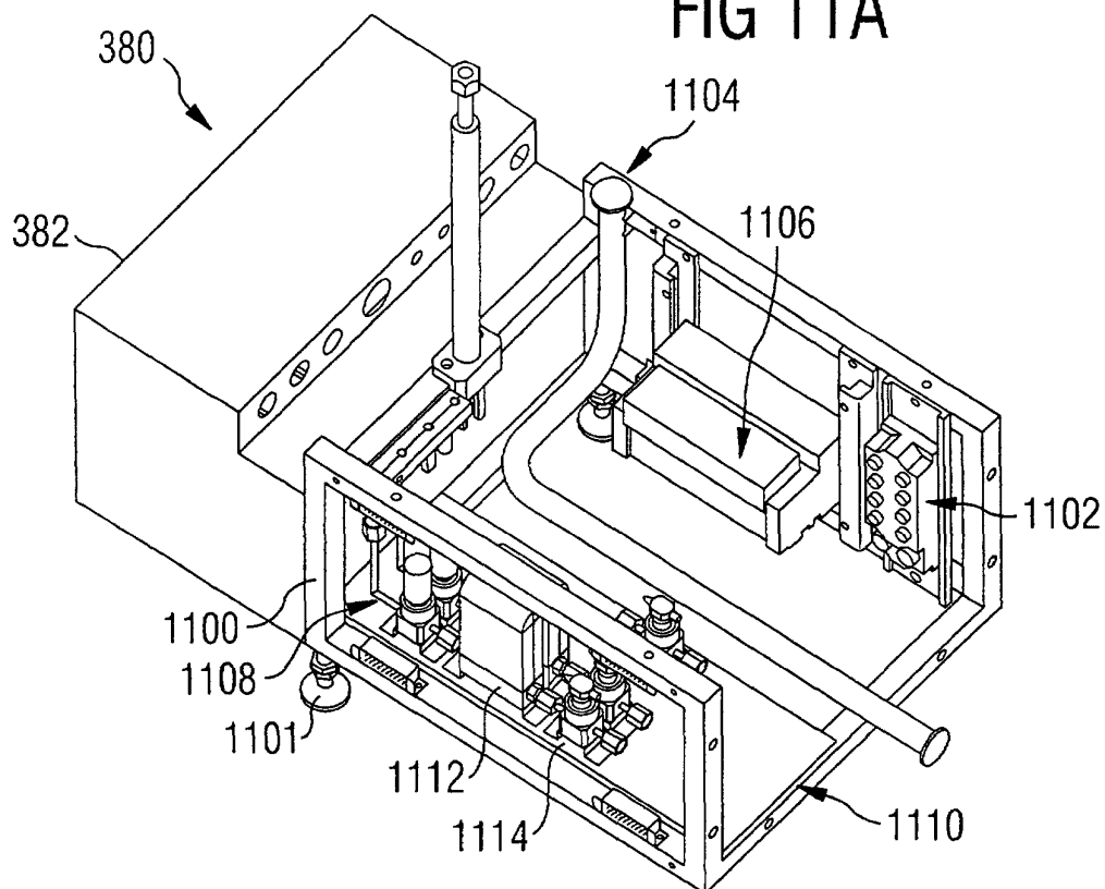
CHAMBER TRAY 3D VIEW
