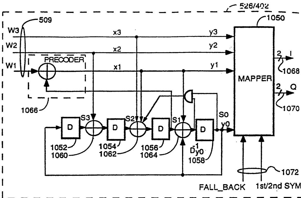
PREFERRED TRELLIS ENCODER
