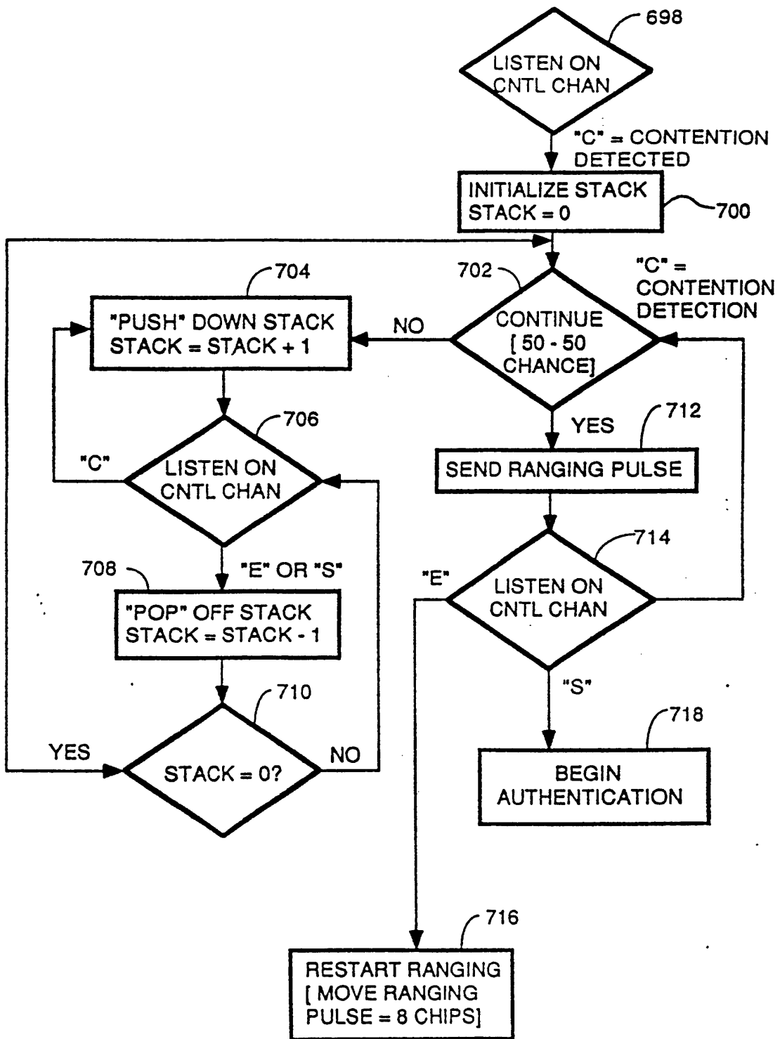
CONTENTION RESOLUTION - RU USING BINARY STACK
