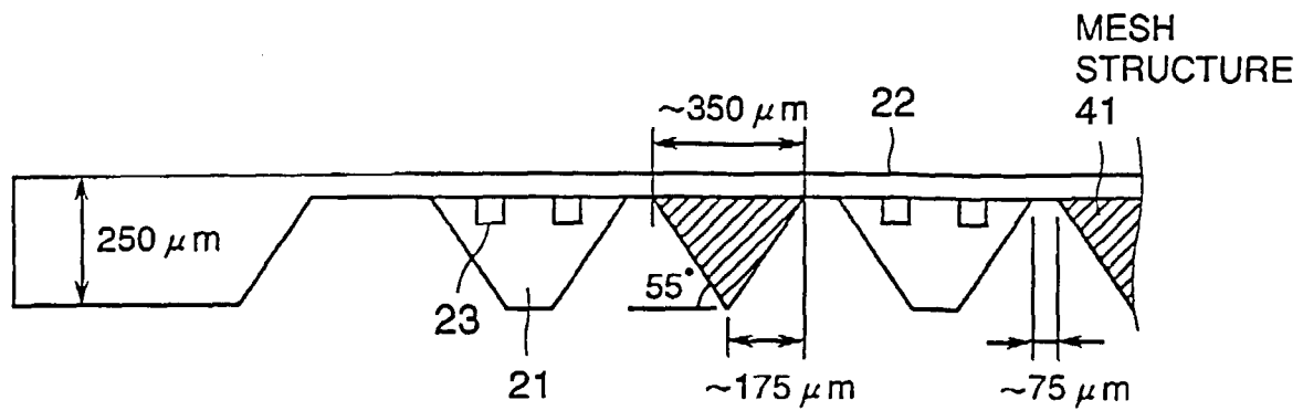
A CROSS SECTION VIEW AT B-B'
