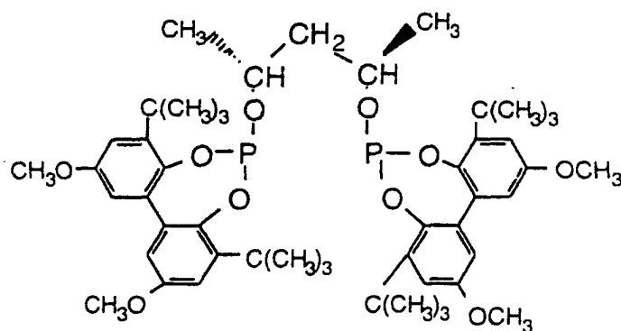
Ligand M
