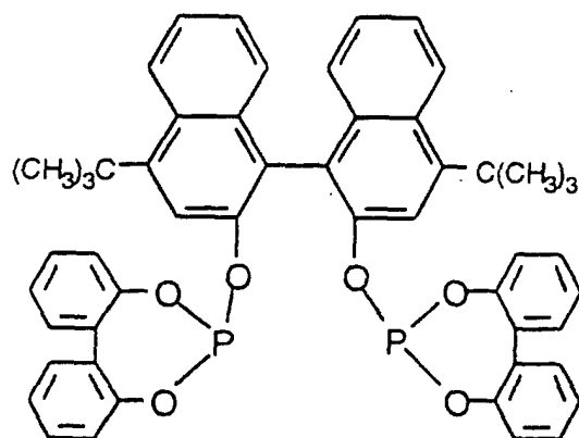
Ligand C
