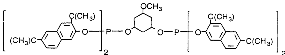
Ligand S
