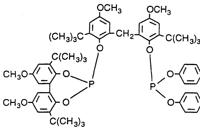
Ligand R
