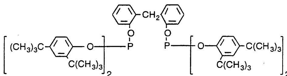
Ligand U
