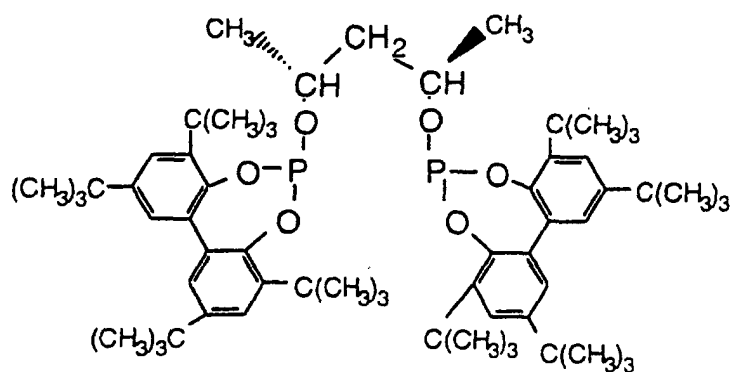
Ligand H
