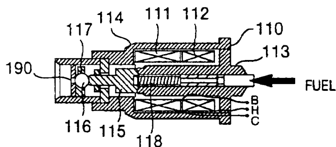
FIG.21A DRAWING OF INJECTOR STRUCTURE
