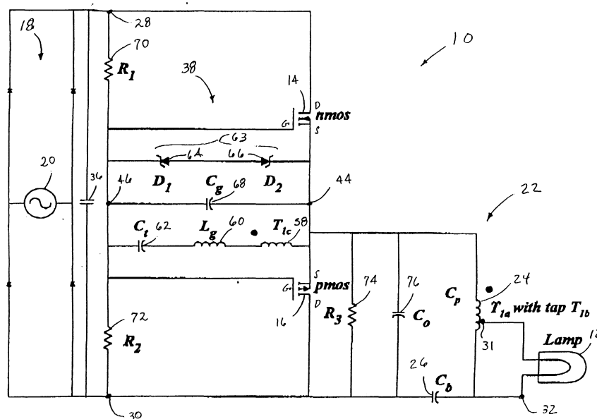
Halogen power converter with complementary transistors.
