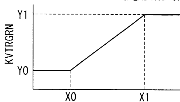
FIG. 7 KVTRGRN TABLE DEPENDING ON VP
