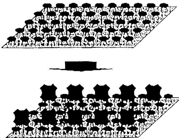
Protein monolayer
