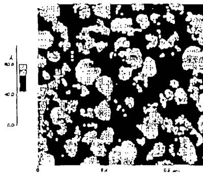
• Gold Substrate
