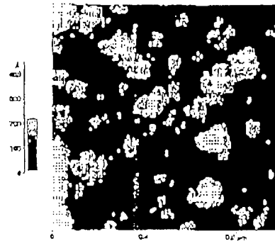
• Antibody monolayer
