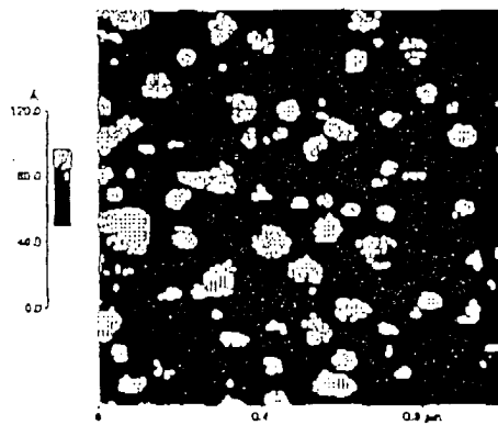
• Gold Substrate
