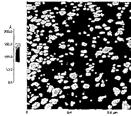
• Antigen monolayer
