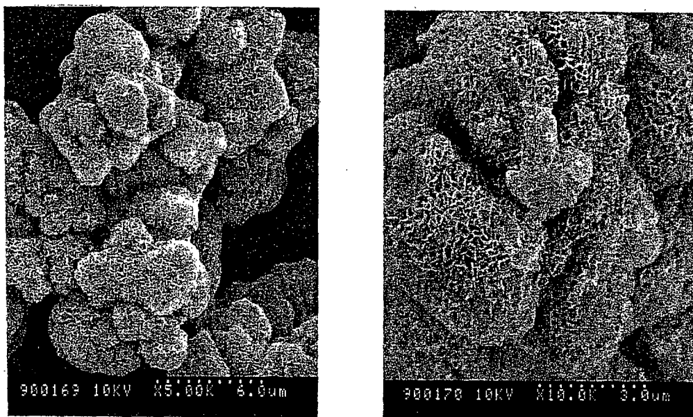
SCANNING-TYPE ELECTRON MICROPHOTOGRAPH OF EX.6.
