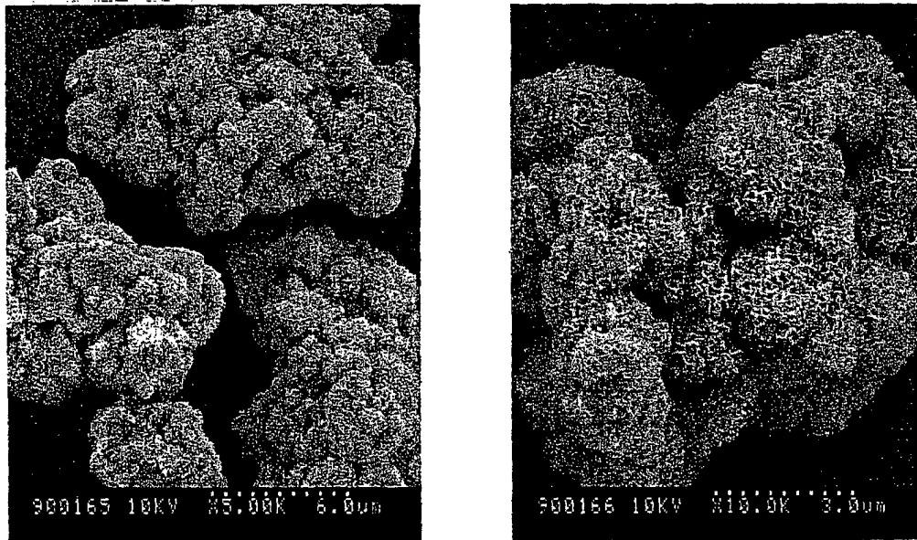
SCANNING-TYPE ELECTRON MICROPHOTOGRAPH OF EX.3.
