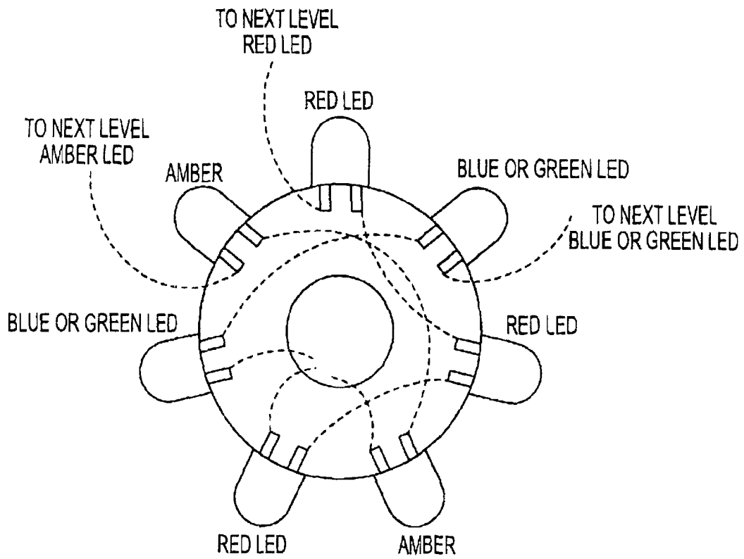
LED WIRING
