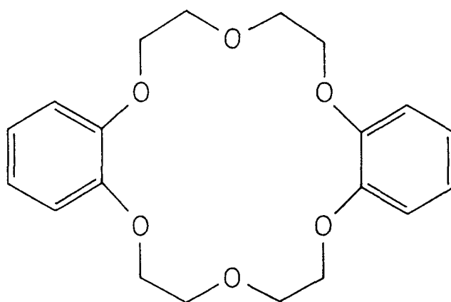
DIBENZOYL-18-CROWN-6
