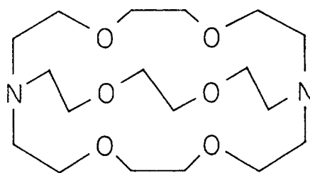
CRYPTAND [2.2.2]
