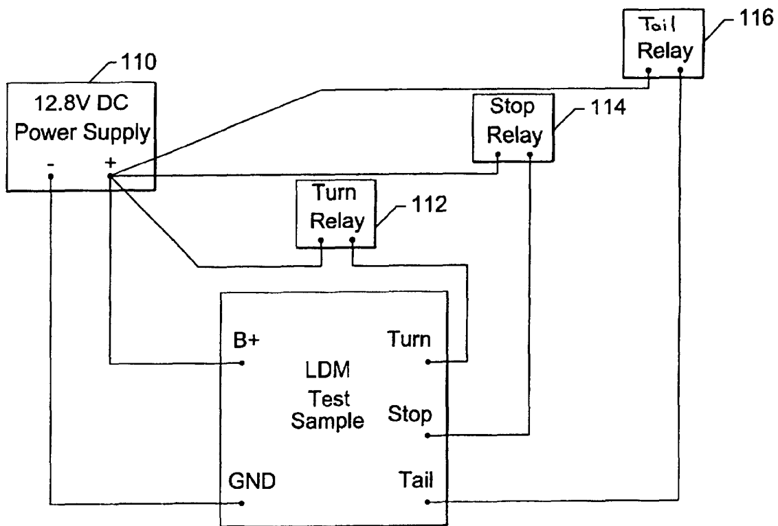
Schematic of life cycle test set up
