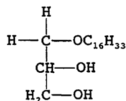
(chimyl alcohol)
