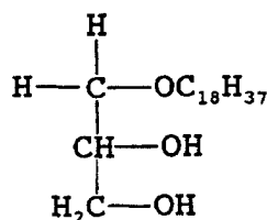
(batyl alcohol)
