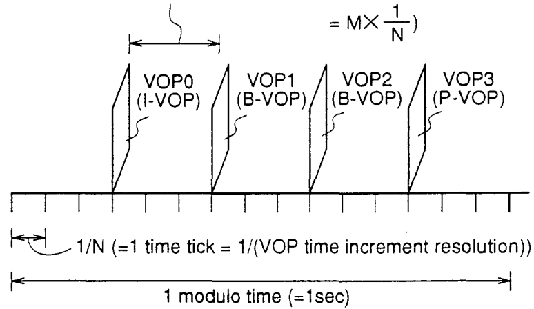
Fig.17 (b) frame cycle (1 fixed VOP increment = VOP rate increment \times time tick
