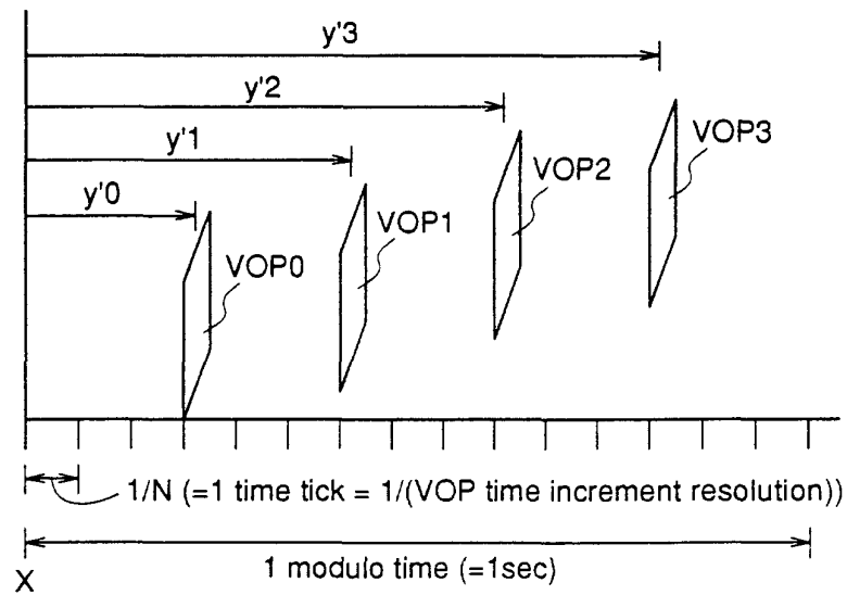
Fig.17 (b) frame cycle (1 fixed VOP increment = VOP rate increment \times time tick
