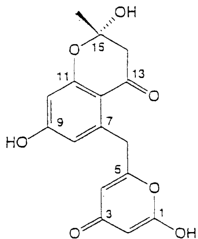
SEK4 ( 12 )
