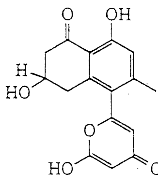
MUTACTIN (6)
