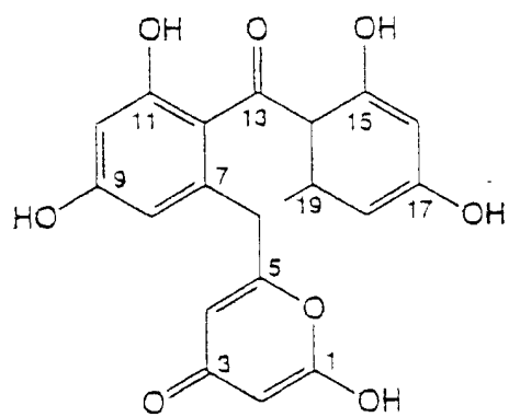
SEK15 ( 13 )
