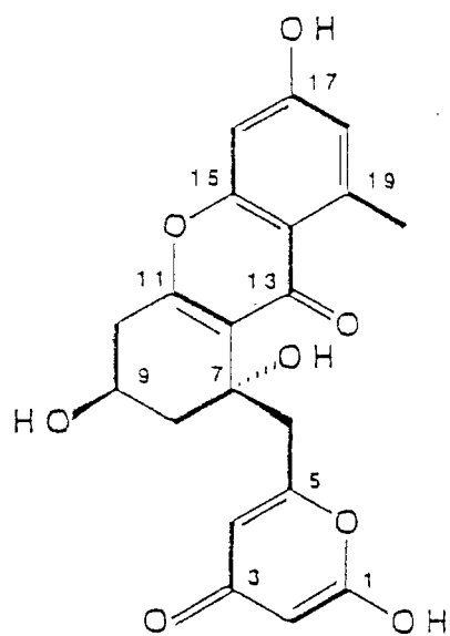
RM20c (15)
