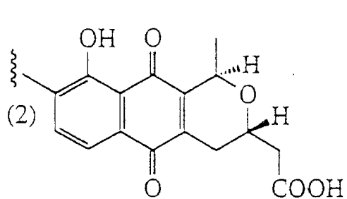
ACTINORHODIN (3)
