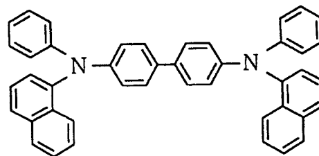
a - NPD
