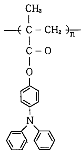
TPA - PMMA
