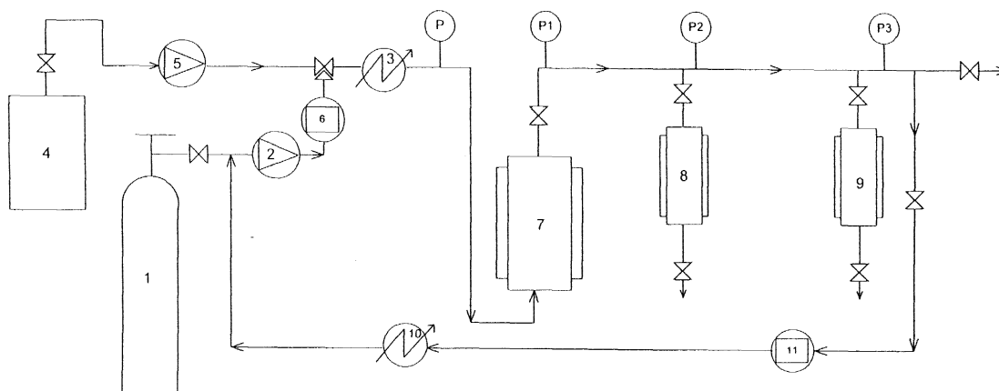
Figure 1 – Flowsheet of the extraction and separation plant.
