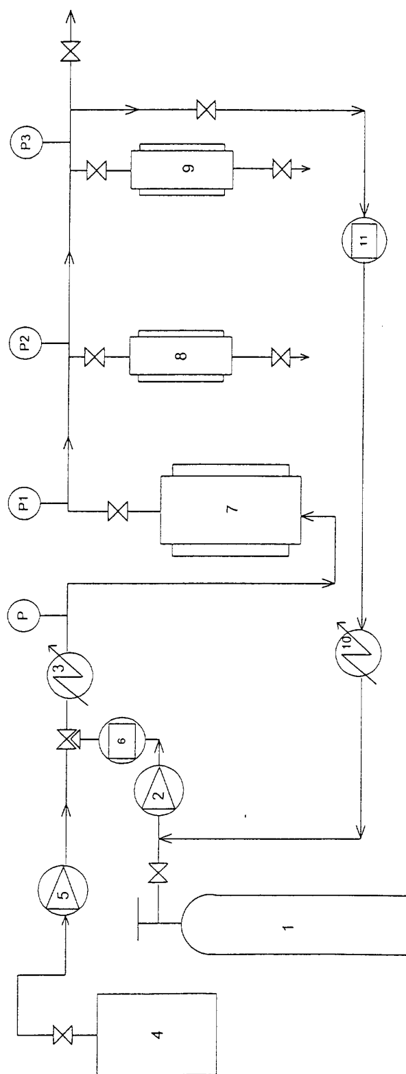
Figure 1 – Flowsheet of the extraction and separation plant.
