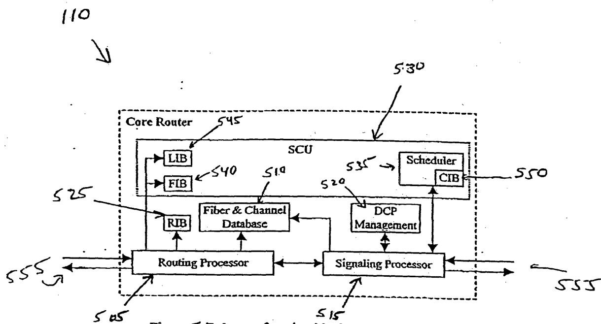
Figure 5. Relevant function blocks at a core router.
