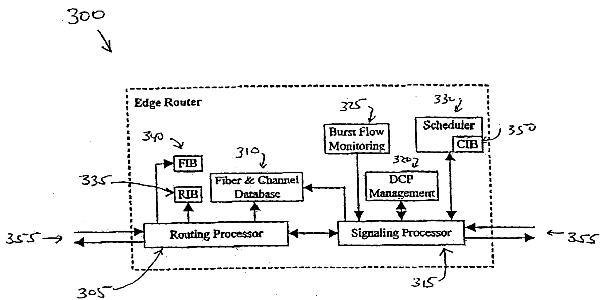
Figure 3: Relevant function blocks at an edge router.
