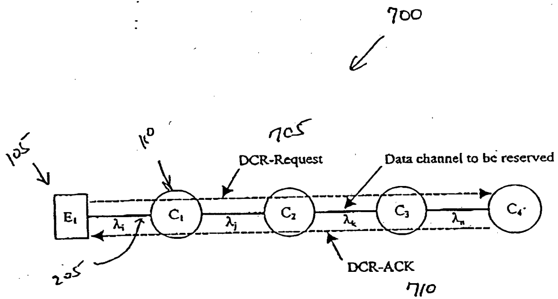
Figure 7 Data channel path setup.
