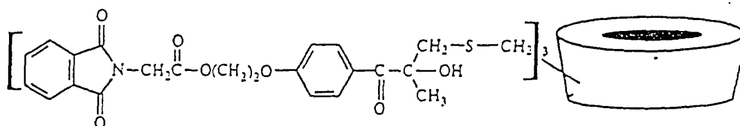
Hydroxy Compound
