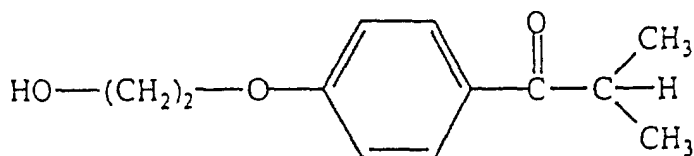
Dehydroxy 2959
