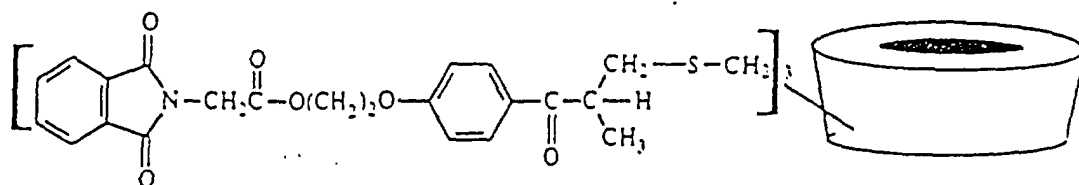
Dehydroxy Compound
