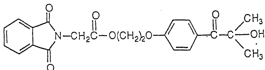
phthaloylglycine-2959
