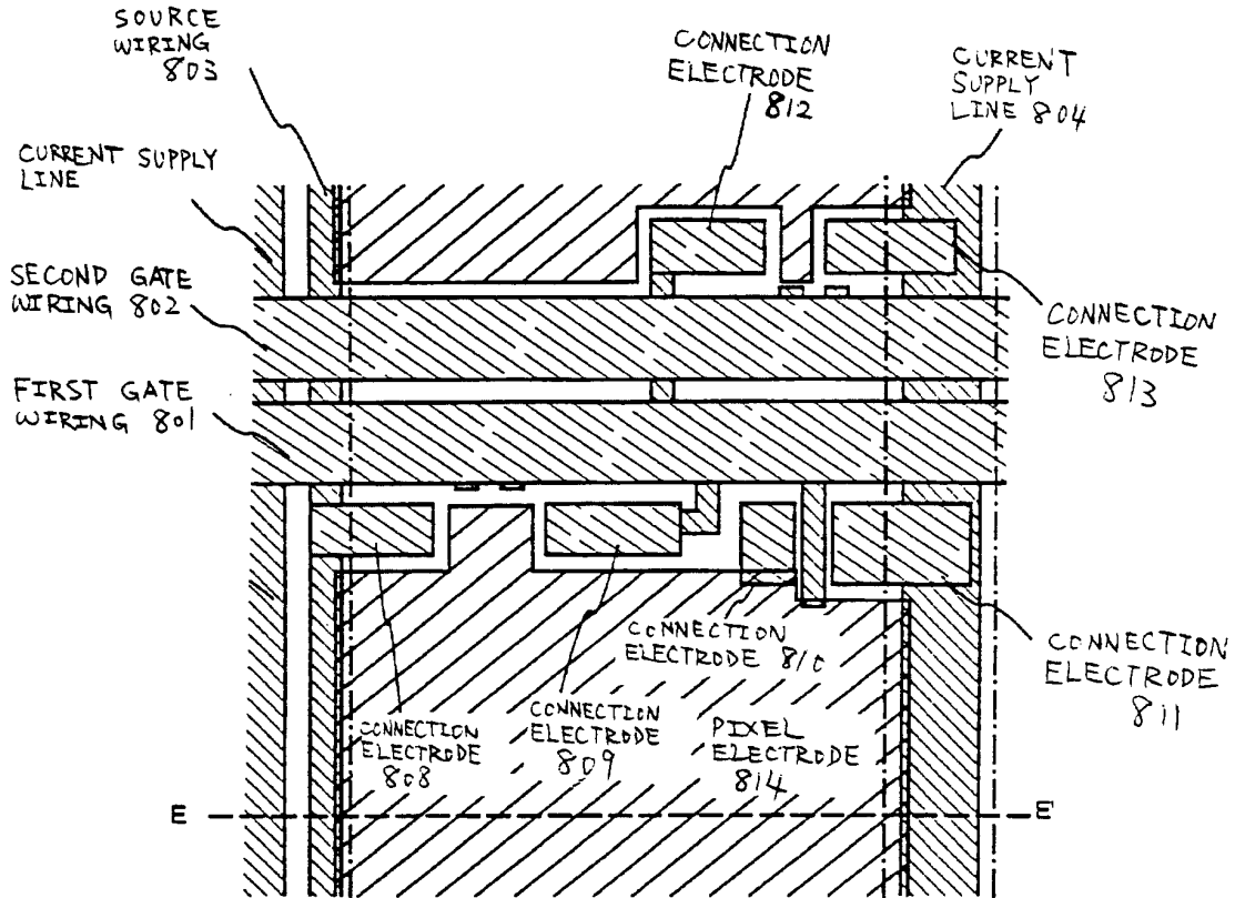
Fig. 10A TOP VIEW
