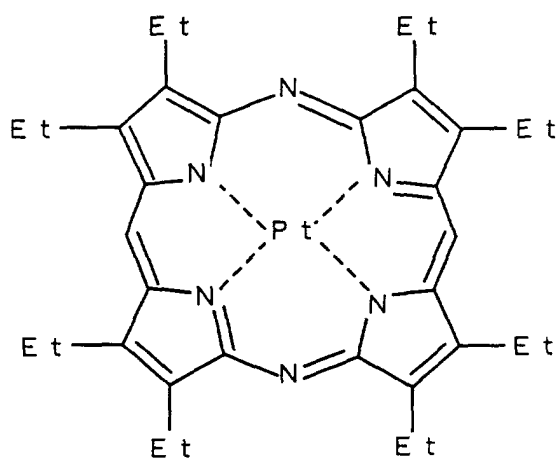
Chemical Formula 7
