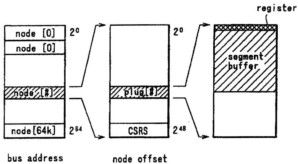
Location of plug address spaces
