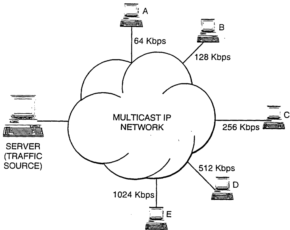
HETEROGENEOUS MULTICAST IP NETWORK (e.g., MBONE)
