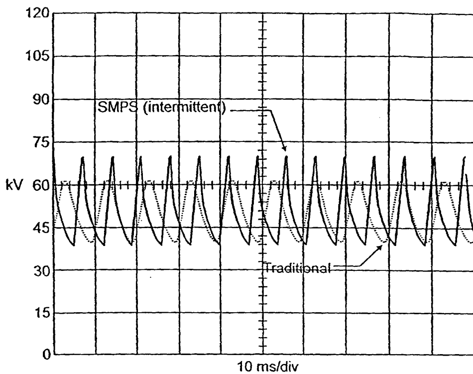
Fig. 3 Waveforms of the precipitator voltage
