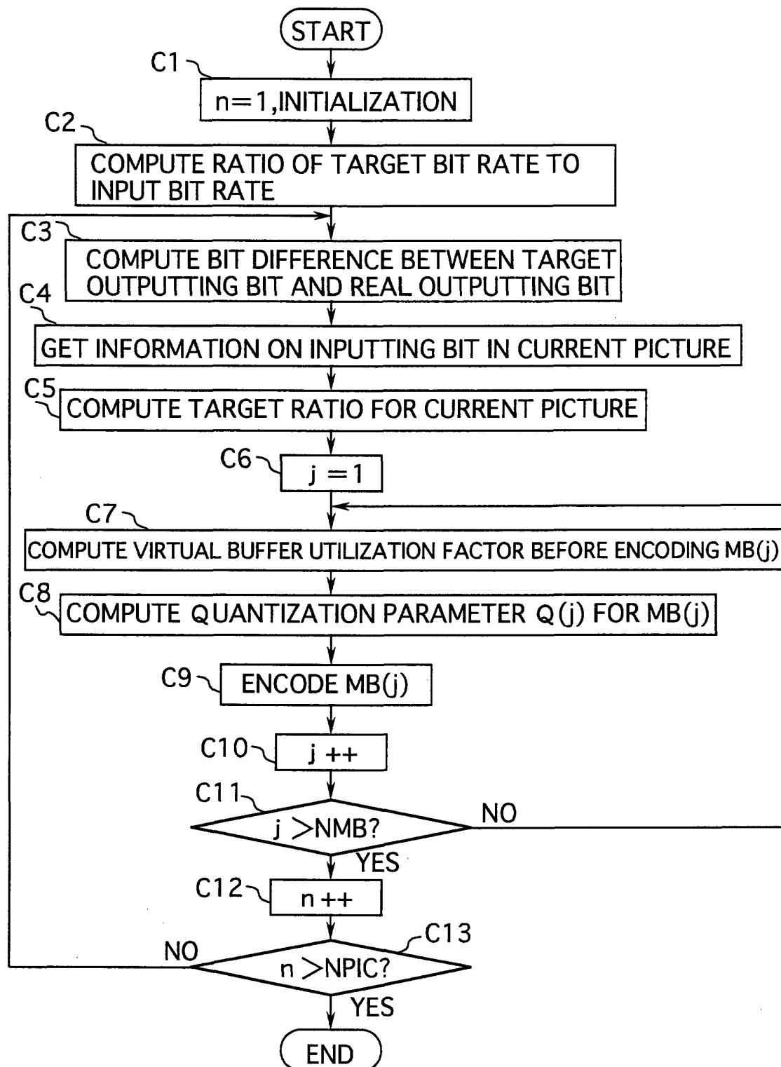
FIG.23 PRIOR ART
