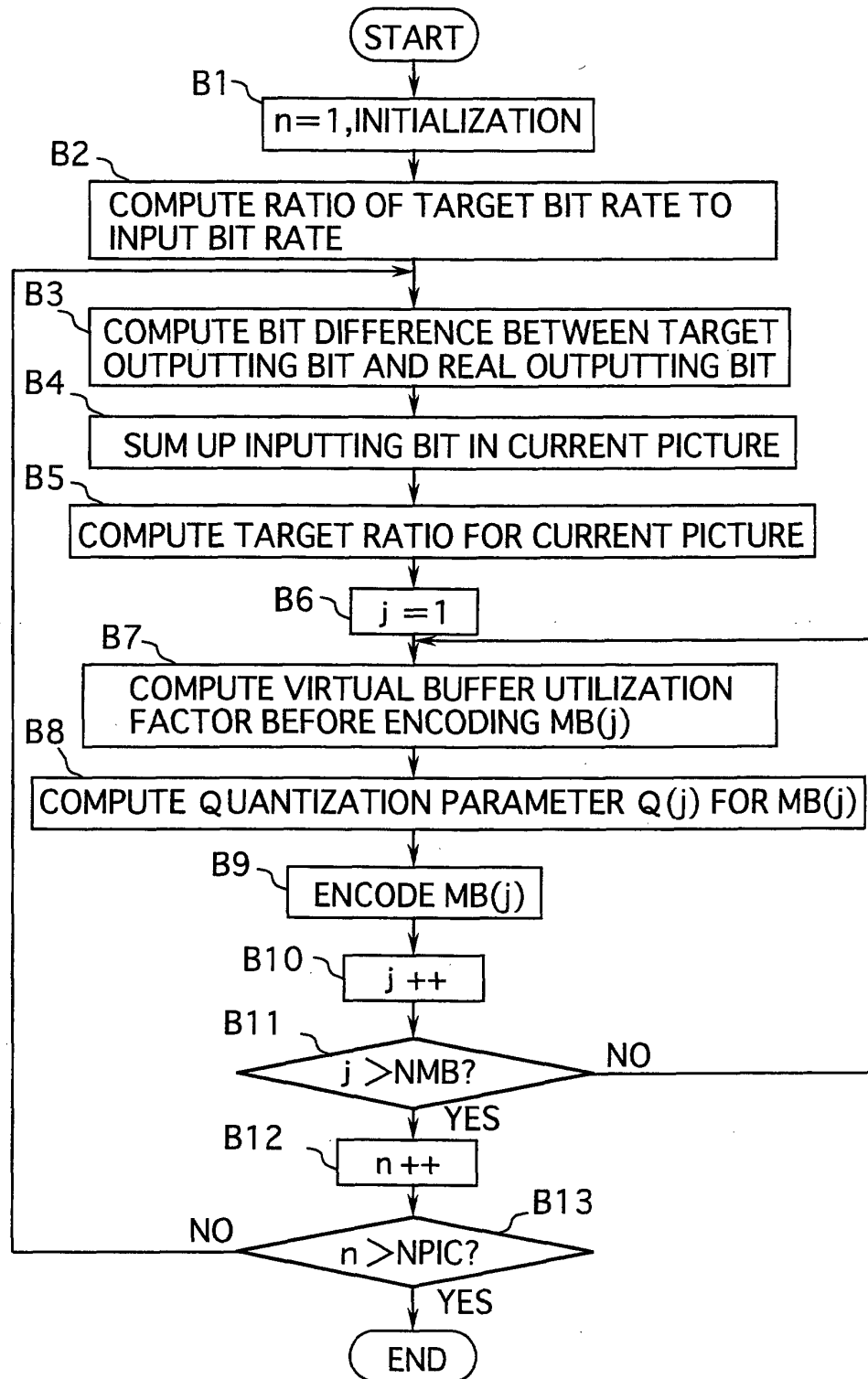
FIG.21 PRIOR ART
