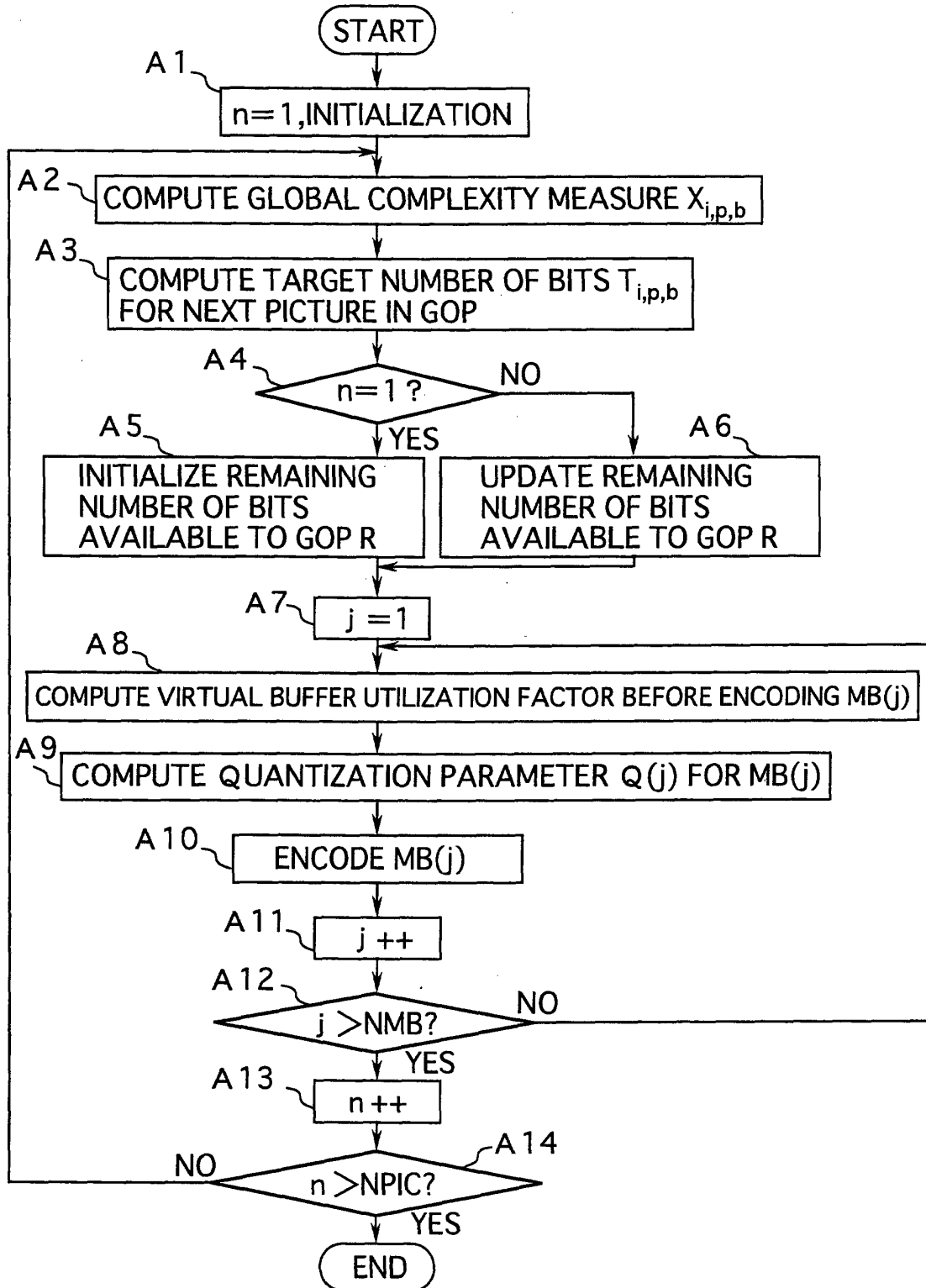
FIG.19 PRIOR ART
