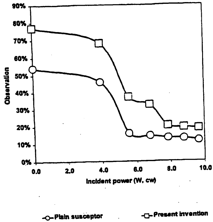
Reflection characteristics
