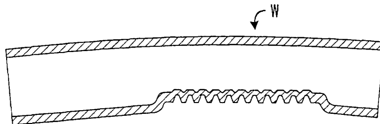
Fig. 5 PRIOR ART
