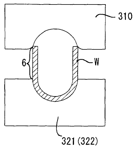
Fig.7c PRIOR ART
