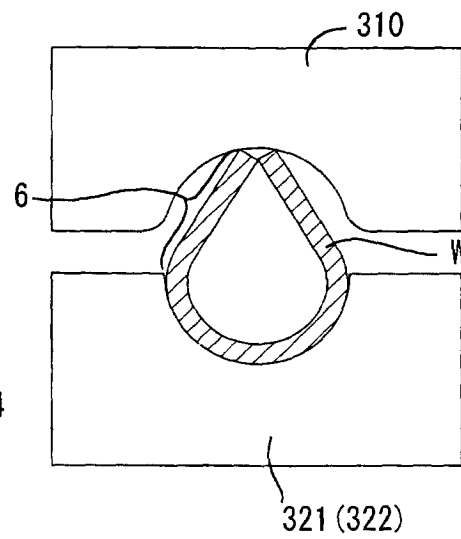
Fig.8c PRIOR ART
