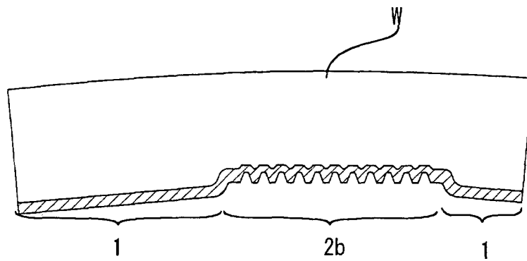
Fig. 4 PRIOR ART
