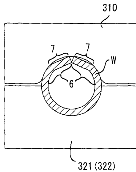
Fig.9c PRIOR ART
