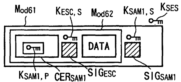
FIG.43I SAM105 1 → 102 (ESC) (IN-BAND)
