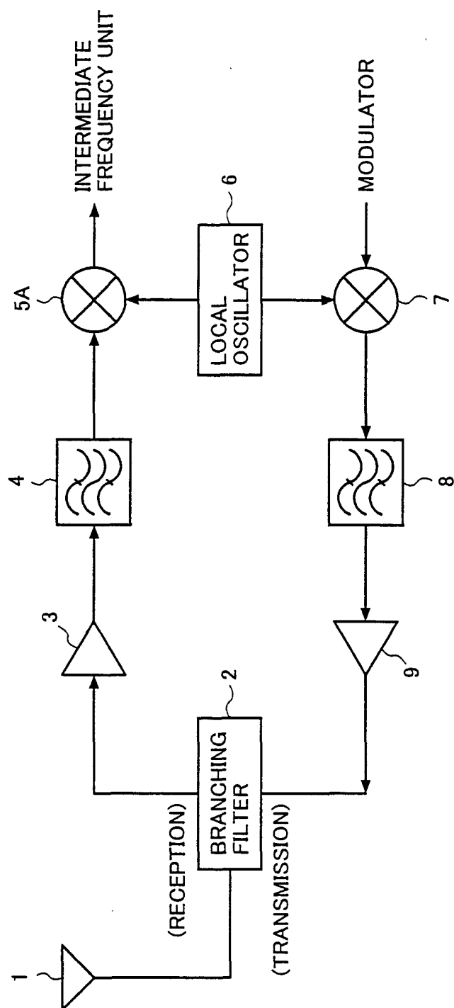
FIG.1 PRIOR ART
