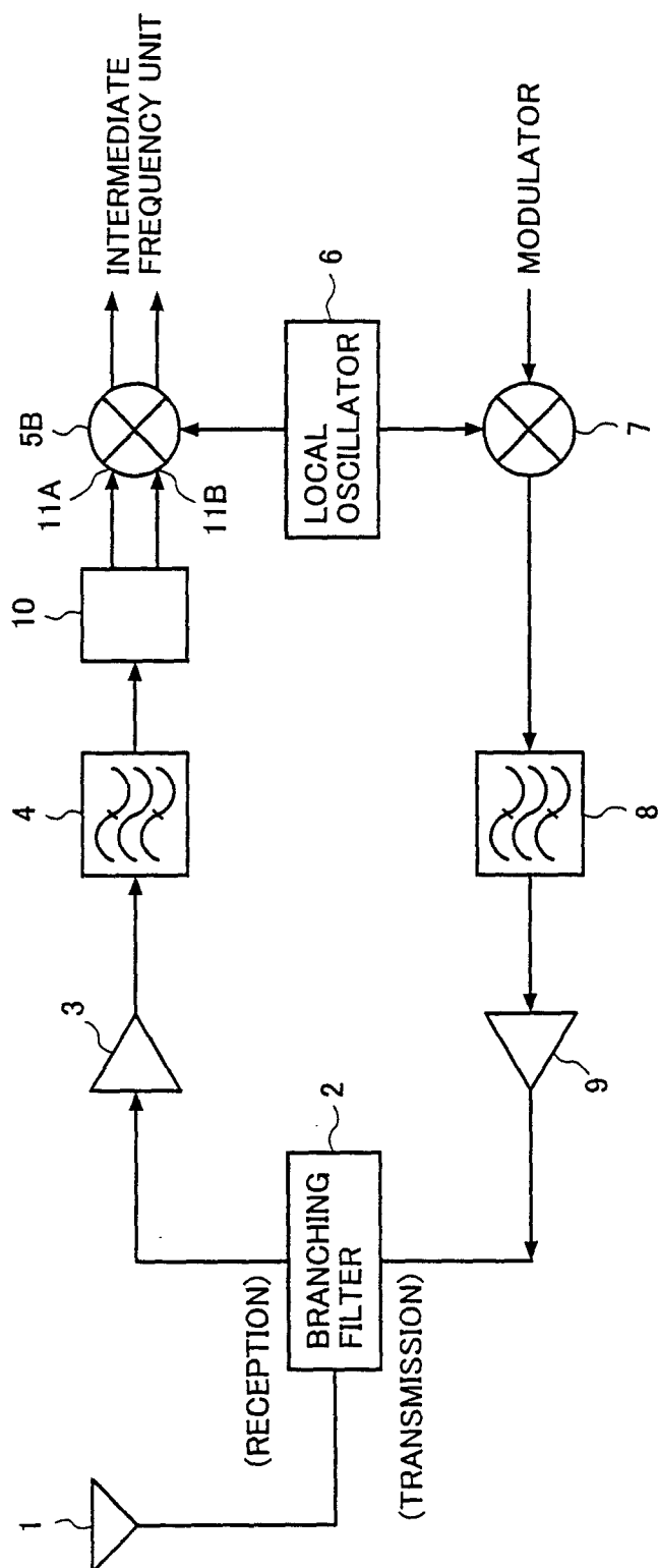
FIG.2 PRIOR ART
