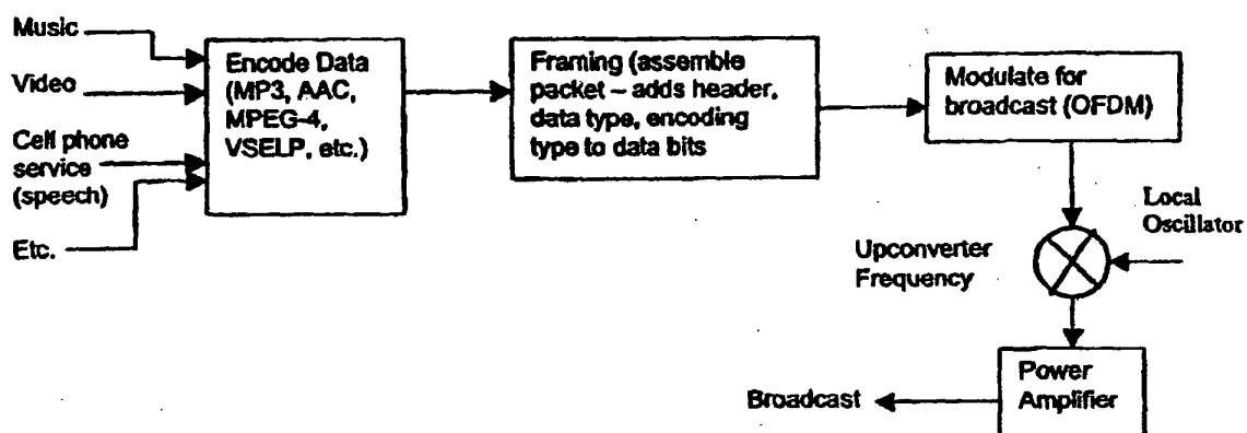
Fig. 28 - Transmitter Architecture
