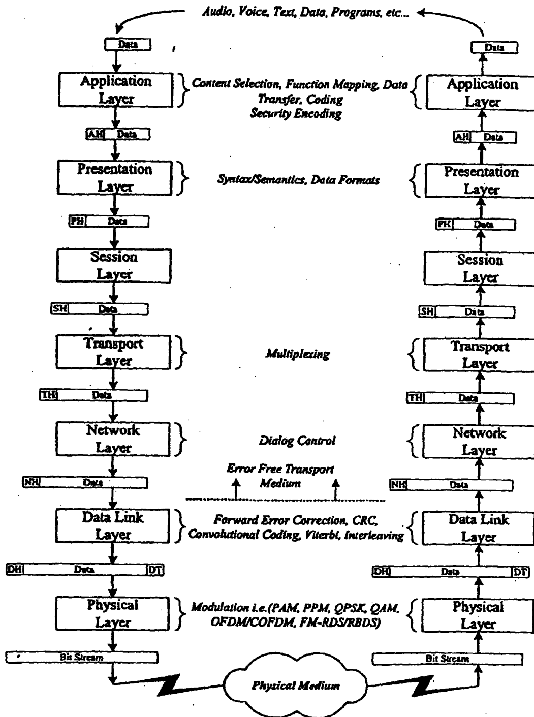
Fig. 30 - Layered Protocol Model
