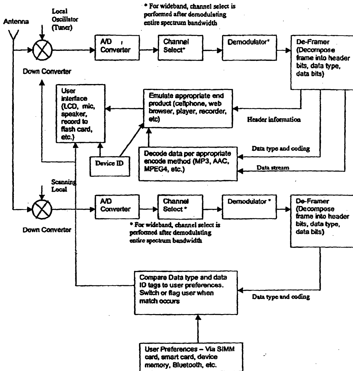
Fig. 29 - Receiver Architecture
